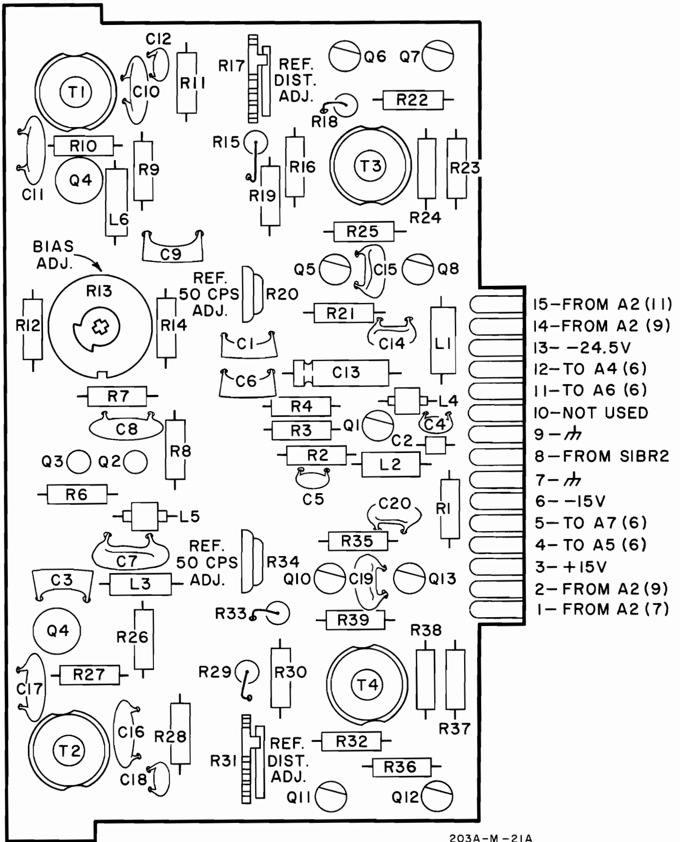
Figure 5-15. Modulator Assy A3--Component Location
