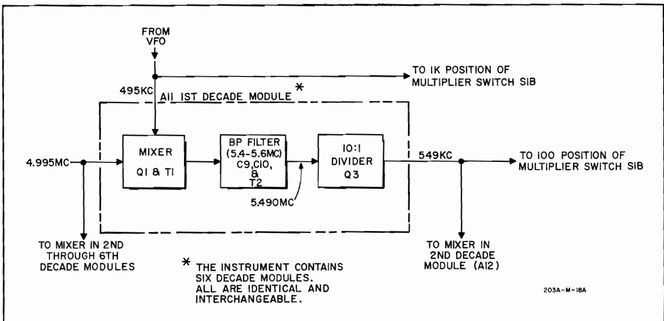
Figure 4-2. Circuit Details
