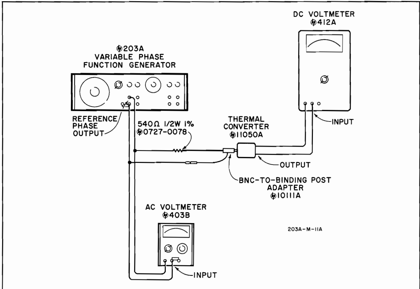
Figure 5-2. Frequency Response
