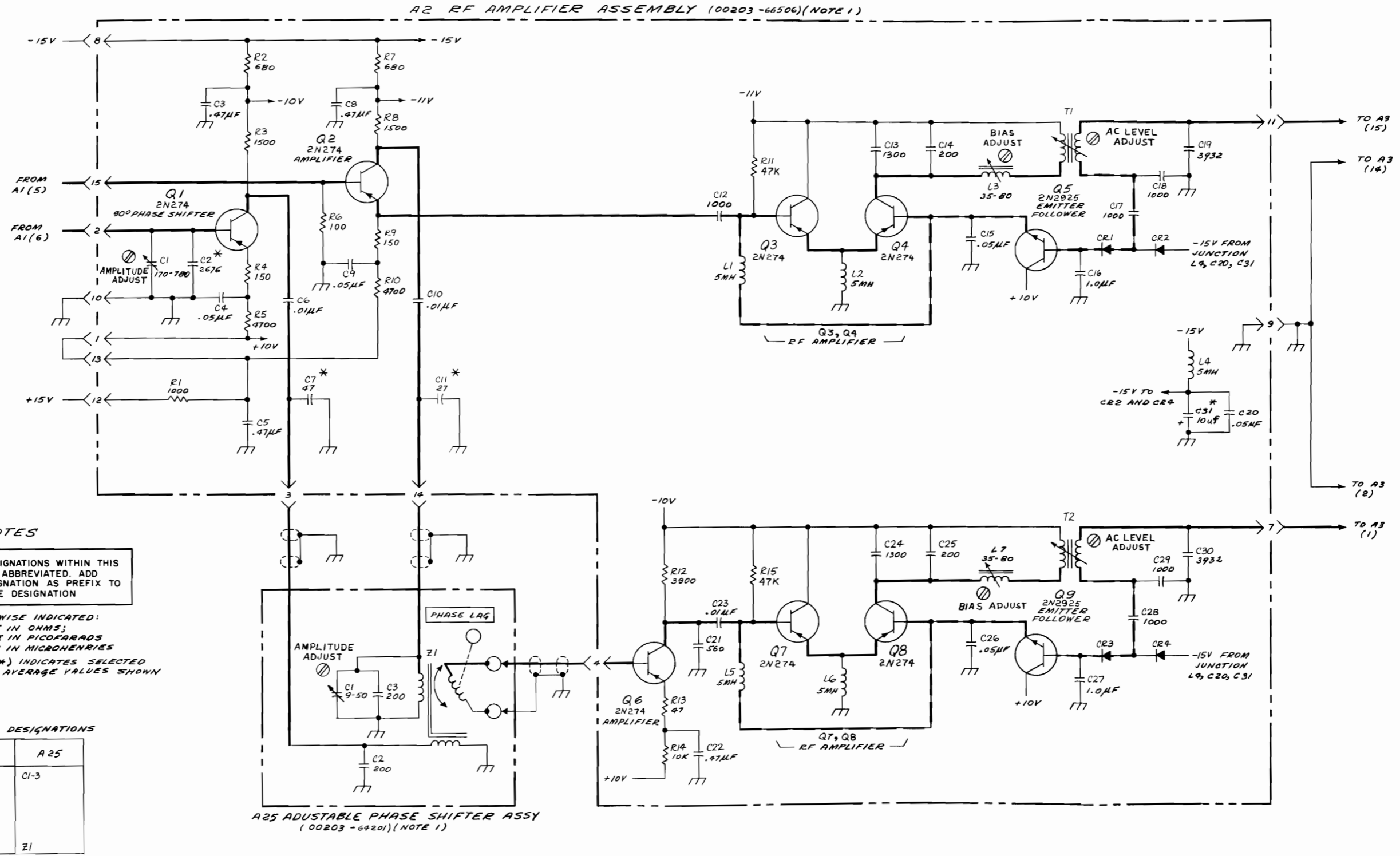
Figure 5-12. RF Amplifier Assy A2 and Adjustable Phase Shifter Assy A25--Schematic
