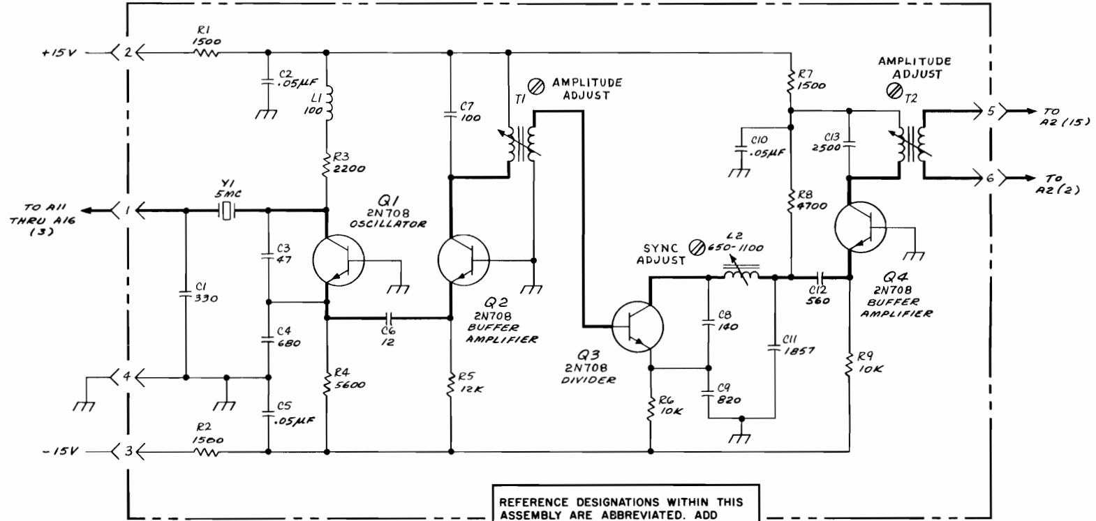
Figure 5-10. 5 Mc Oscillator and 9:1 Divider Assy A1--Schematic
