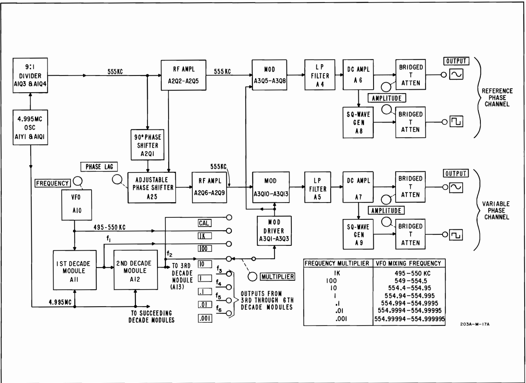
Figure 4-1. Block Diagram
