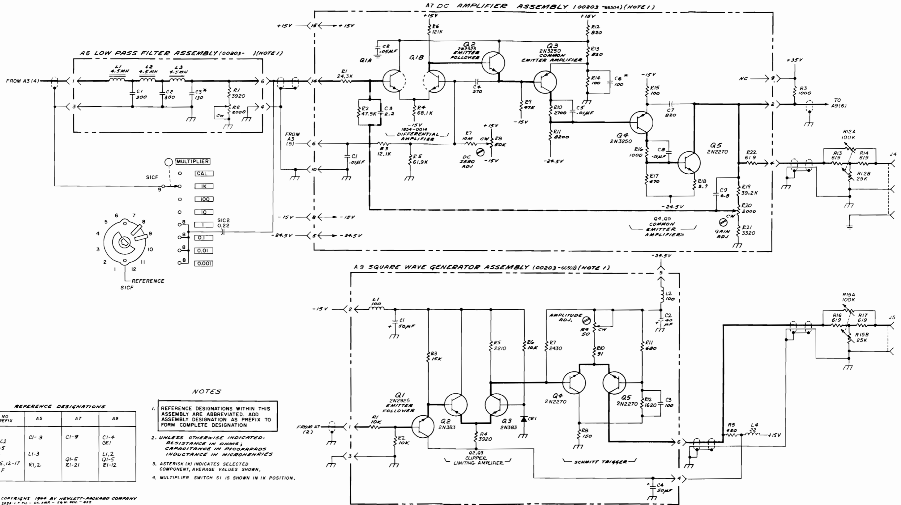
Figure 5-20. Low Pass Filter Assy A5, DC Amp Assy A7, and Square Wave Gen Assy A9--Schematic
