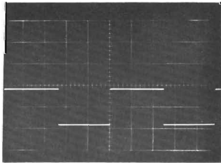
18- A8Q4 Collector FREQUENCY - 1 kc 5 V/CM; .2 \mu SEC/CM
