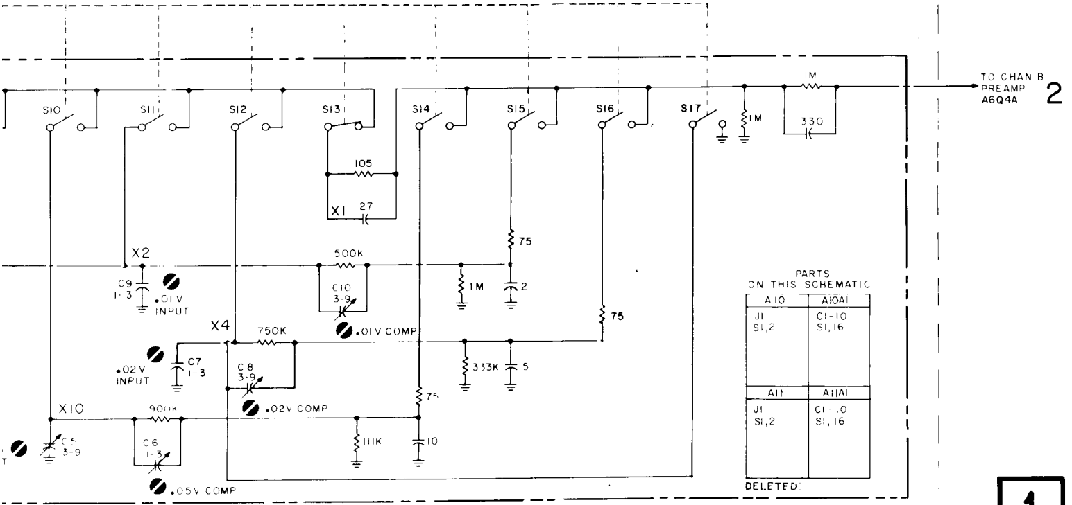
Figure 8-5. Attenuator Schematic 8-9
