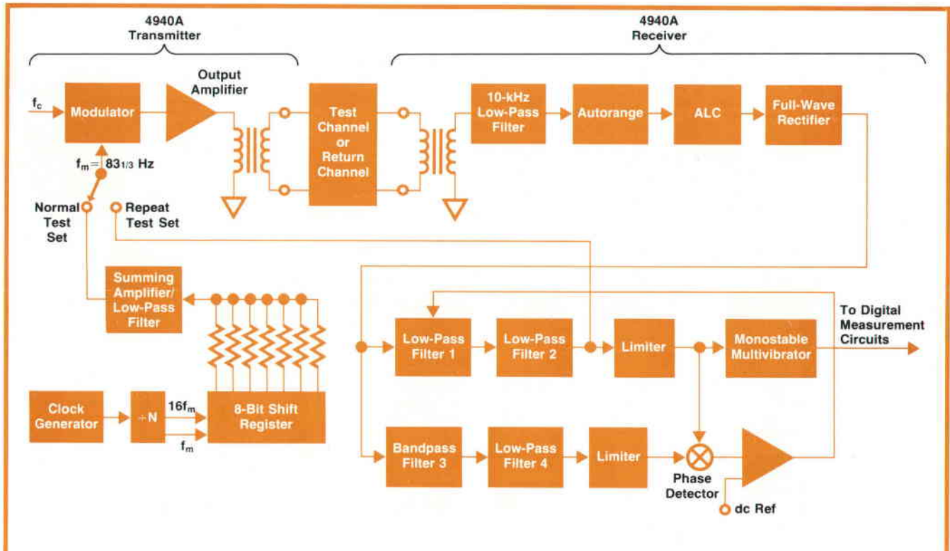
Fig. 2. 4940A envelope delay transmitter and receiver circuits
