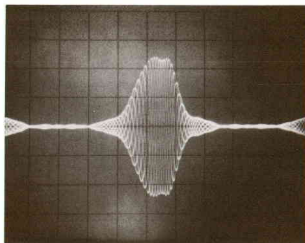
Fig. 1. Frequency spectrum and envelope of transmitted signal for peak-to-average ratio measurements.
