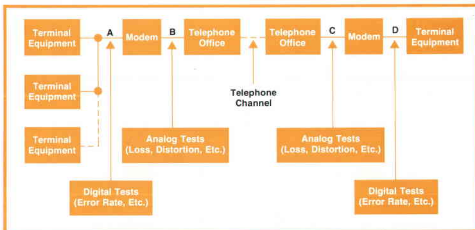
Fig. 1. A general data network, showing where analog and digital test instruments are used.
