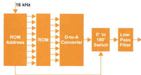
Fig. 2. P/AR signal waveform is stored in a read-only memory in the 4940A. This method of generation allows the receiver to be much less complex and expensive than previous methods.
