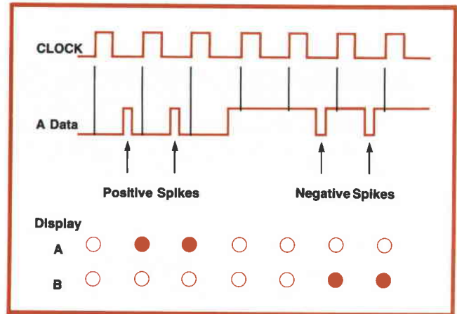
Fig. 5. Spikes occurring between clock pulses may be desired signals or noise. In SPIKE A mode, the Analyzer displays spikes and shows whether they are positive-going or negative-going.
