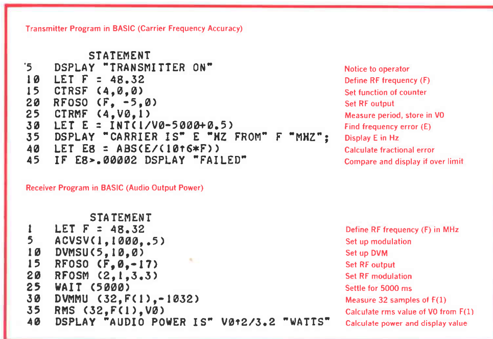
Fig. 6. Sections of typical test programs written in ATS BASIC.
