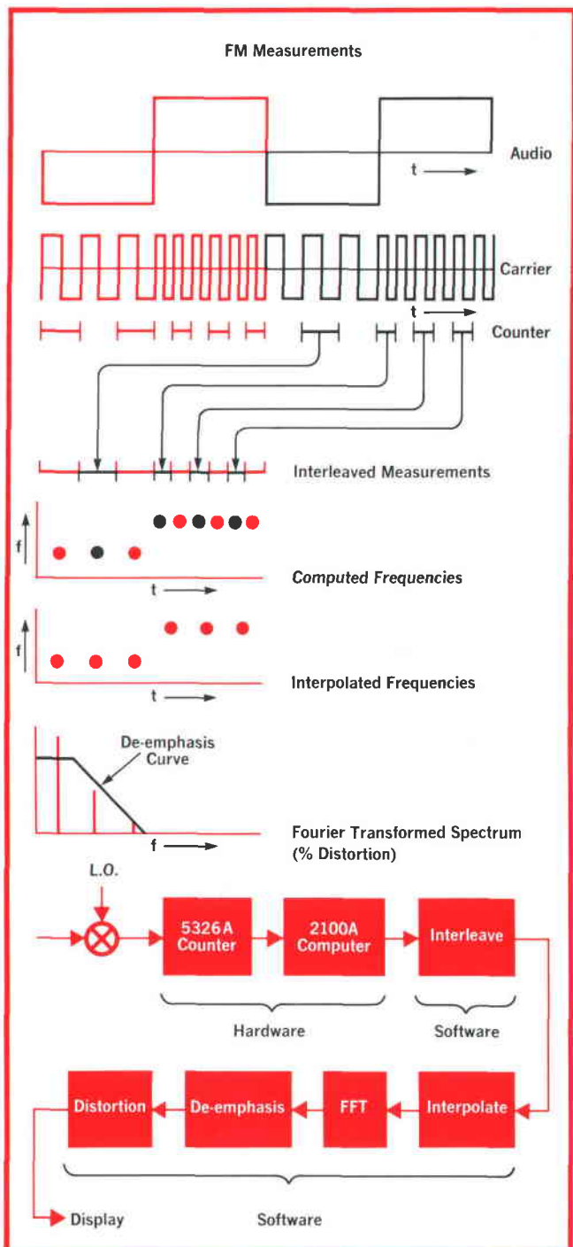
Fig. 3. In FM measurements the counter, acting as a frequency-to-digital converter, measures every other carrier period over two modulation cycles. These measurements are interleaved and a set of equally-spaced frequency samples is computed. These are transformed to derive the spectrum and determine distortion.
