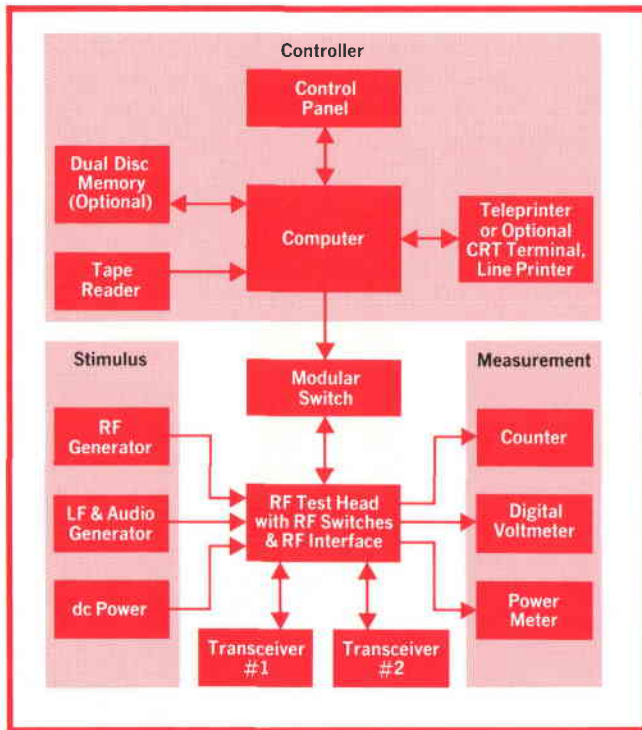
Fig. 3. Transceiver stimulus is provided by a signal generator and a frequency synthesizer. Measurements are made by a multimeter, a counter, and a power meter, supplemented by special software to compute distortion and other parameters. A modular switch sets up measurement paths under computer control.
