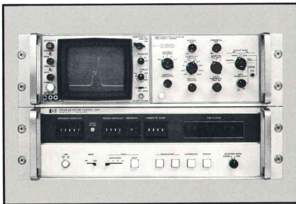
Fig. 10. Range of energies to be scanned, the starting energy, the scan rate, and the number of scans are selected at the detector control unit. The multichannel analyzer displays the resulting spectrum. Data can also be plotted or transmitted to a computer for analysis.
