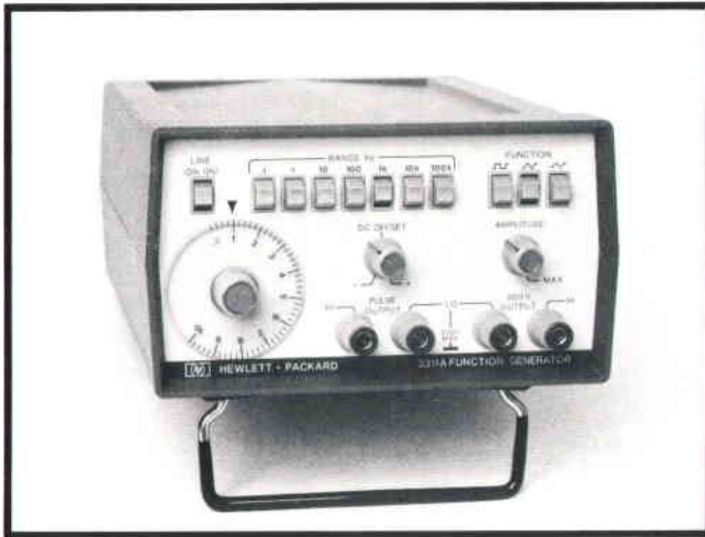
Fig. 2. New Model 3311A Function Generator supplies waveforms for many kinds of tests over 0.1 Hz to 1 MHz frequency range. Maximum output is 10V peak to peak into a 600 \Omega load (20V into an open circuit). The amplitude control has a range of 30 dB.
