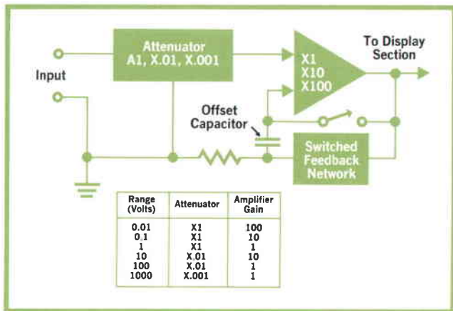
Fig. 2. In voltmeter mode, attenuator and amplifier scale input to voltage between -1.99999 and +1.99999 for digital presentation by Display section.
