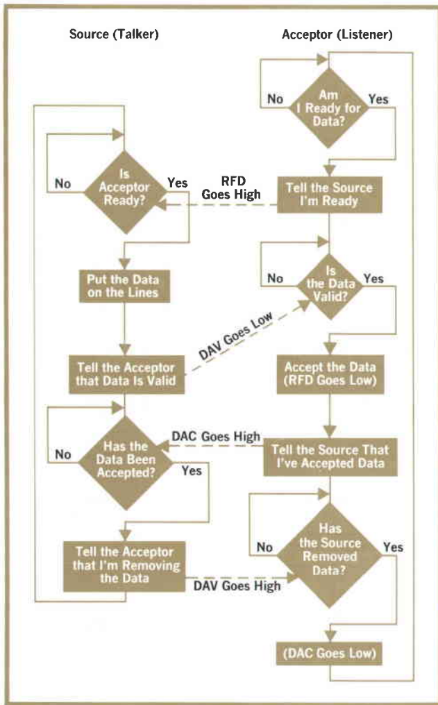
Fig. 3. Flow diagram outlines sequence of events during transfer of data byte. More than one listener at a time can accept data because of logical-AND connection of RFD and DAC lines (see Fig. 4).
