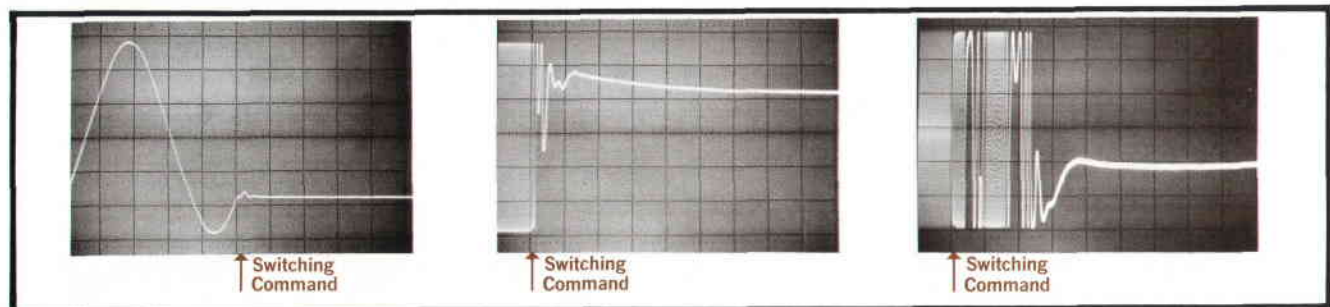
Fig. 5(a). Photo above shows small transient as Synthesizer switches from 10.00099 MHz to 10.00000 MHz, a full-range transition for PLL3 (10 MHz has been subtracted from Synthesizer output to clarify presentation).
