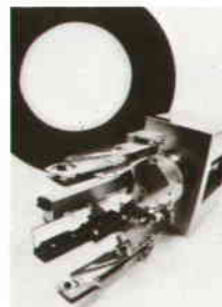
Cover: This is the fast, precise linear-motor actuator and head-carriage assembly that moves the read/write heads in Model 7900A Disc Drive. The upper set of heads is for the removable cartridge and the lower set is for the fixed disc.
