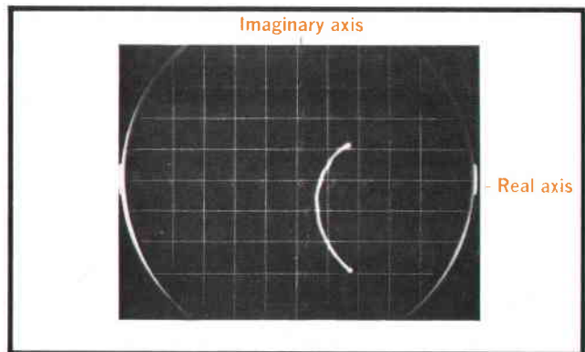
Fig. 3. Impedance of folded dipole antenna over 88-108 MHz frequency range as displayed on Cartesian coordinates with Model 8414A Polar Display. Full scale is 1000\Omega . At 88MHz (lower bound of trace) antenna impedance reads as 350-j600\Omega .
