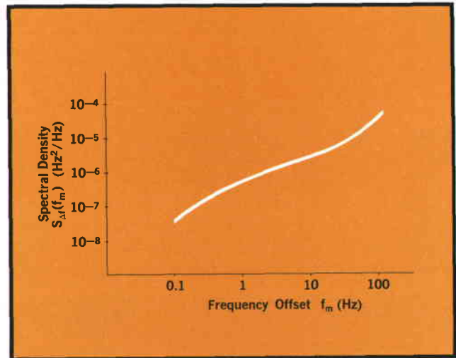
Fig. 6. Spectral density of 500 kHz voltage-controlled oscillator as measured by the setup of Fig. 5.
