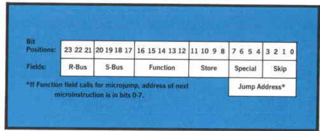
Fig. 4. 24-bit, three address microinstructions are more powerful than the 16-bit user instruction set they are designed to implement. Format of microinstructions makes microprograms easy to write.
