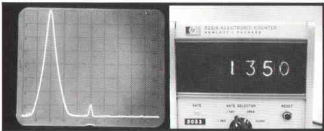
Fig. 5. A 0.3\text{ }\mu\text{V} ( -130\text{ dBV} ) signal is measured only 150 Hz away from a signal 70 dB larger. A counter connected to the tracking generator output was used to measure the frequency of the small signal.
