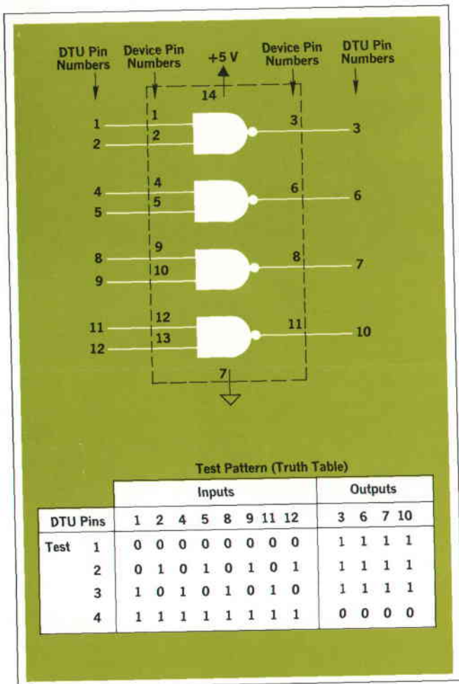
Fig. 3. A simple quad NAND gate to be tested. Test program is explained in text. Digital devices to be tested can have as many as 240 pins.
