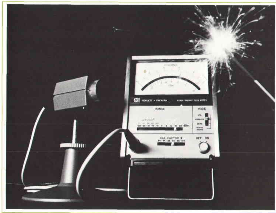
Fig. 1. Easy-to-use, low-cost HP 8330A/8334A Radiant Flux Meter System measures optical power in the ultraviolet, visible, and infrared regions of the electromagnetic spectrum. It reads directly in absolute radiometric units without spectral calibration curves. Maximum absolute uncertainty is less than \pm 5\% of full scale.
