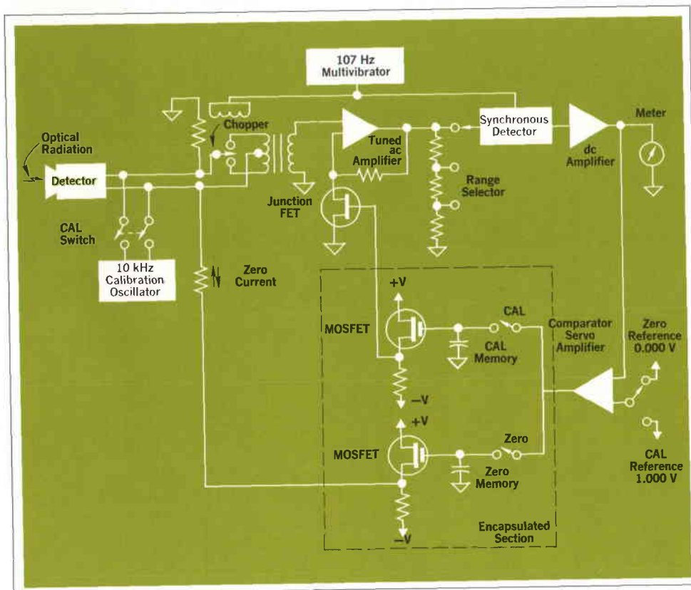
Fig. 5. Sensitive, low-noise input amplifier doesn't degrade detector characteristics. Automatic zero system suppresses background radiation. Automatic calibration system eliminates time-consuming calibration against external standards and increases user confidence.
