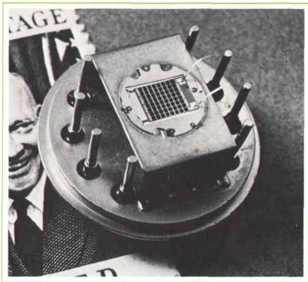
Fig. 2. Unique, HP-designed thin-film thermopile detector has fast five-millisecond response, low drift, and high immunity to mechanical shock.
