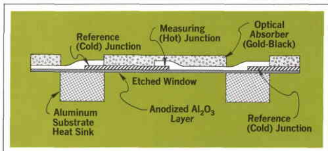
Fig. 3. Thin-film thermopile consists of 64 antimony-bismuth thermocouples connected in series.
