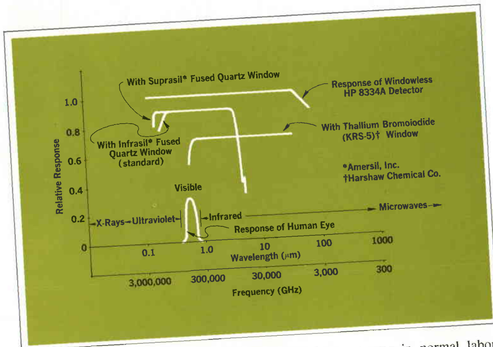
Fig. 4. Flat response of detector allows accurate broadband measurements. Spectral range varies with transmission characteristics of window mounted in front of thermopile.
