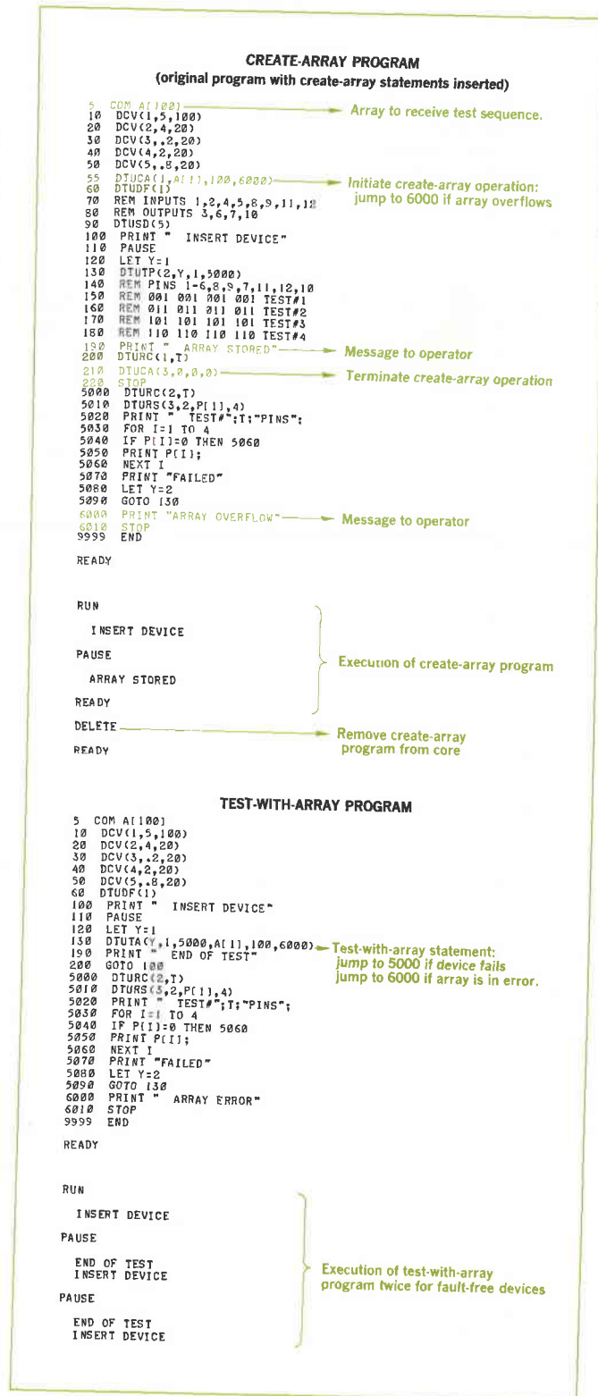
Fig. 4. Test pattern created and checked out in interactive mode is stored in compiled form by inserting 'create array' statements in program. Tests run much faster in compiled mode: for a 12-pin device maximum test rates are approximately 22,000 tests per second in compiled mode and 150 in interactive mode.
