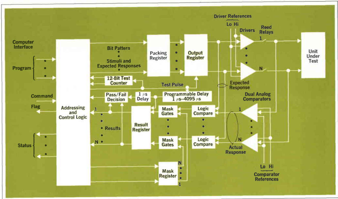
Fig. 2. The digital test unit contains driver and comparator circuits for every pin. Input and output pins are specified in the BASIC program and no hardware changes need be made.
