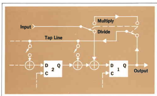
Fig. 9. Data stream introduced into shift register through modulo-2 input is divided by characteristic digital equation of shift register. When data is introduced into tap line, it is then multiplied by shift register equation.
