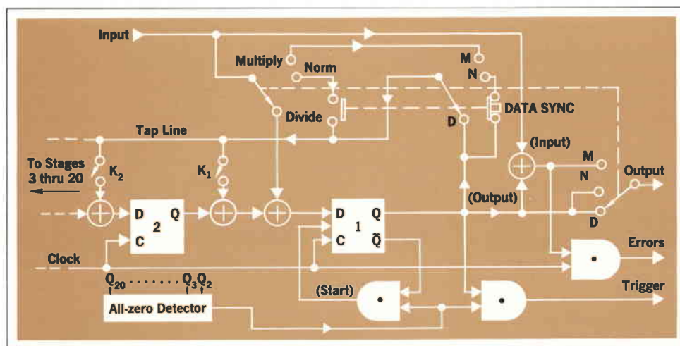
Fig. 10. Simplified block diagram of Model 1930A PRBS Generator.
