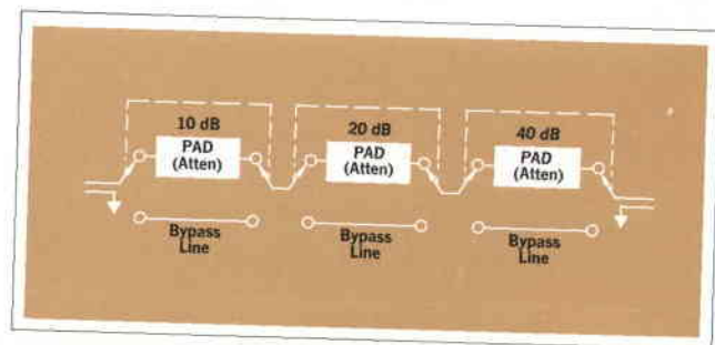
Fig. 1. Circuit arrangement of a cascaded type of step attenuator variable in 10 dB steps from 0 to 70 dB.
