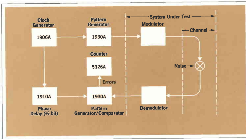
Fig. 3. Loop-around test of digital data transmission system uses one 1930A to generate test pattern and one 1930A to detect transmission errors (see text). Counter measures error rate. Delay Generator shifts phase of clock pulses to prevent overlap with incoming pulse transitions.
