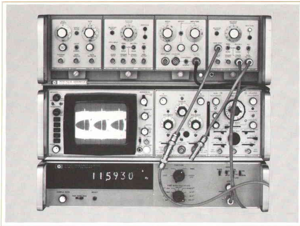
Fig. 1. Model 1930A PRBS Generator is a ¼-width plug-in for Hewlett-Packard 1900-series modular Pulse Generators. 1900 system allows selection of rate generators, delay generators, and pulse amplifier and shaping modules to match 1930A capabilities to wide variety of tasks.
