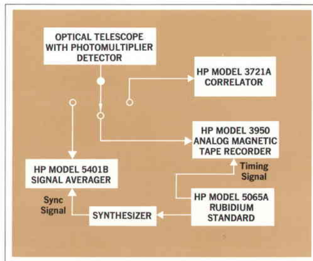
Fig. 1. Block diagram of instrumentation at Lick Observatory for pulsar measurements.
