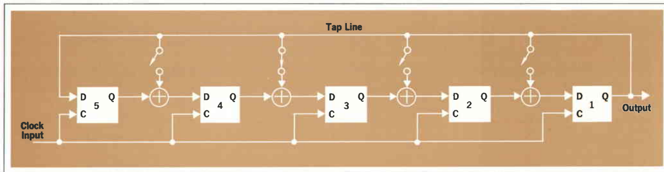
Fig. 8. Shift register configuration that facilitates full control of feedback configuration. This one generates patterns identical to patterns generated by circuit of Fig. 5.
