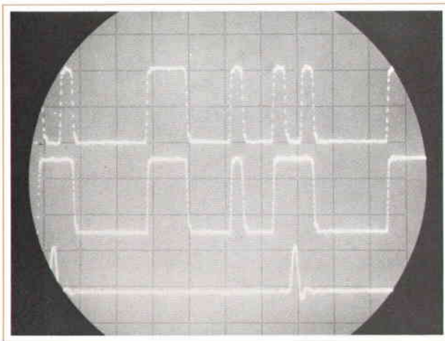
Fig. 2. Model 1930A generates error pulse (bottom trace) whenever input data stream (top trace) differs from internally-generated sequence (center).
