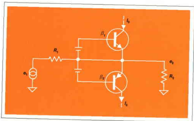
Fig. 1. Two transistors of different \beta feed common load.
