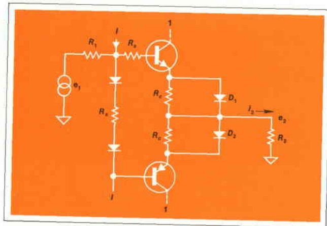
Fig. 7. Diodes shunt R_c to avoid wasting power in resistors.
