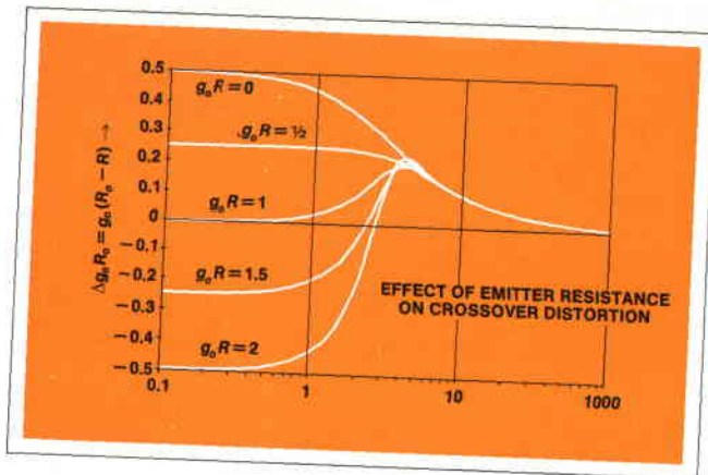
Fig. 6. Effect of emitter resistance on crossover distortion.
