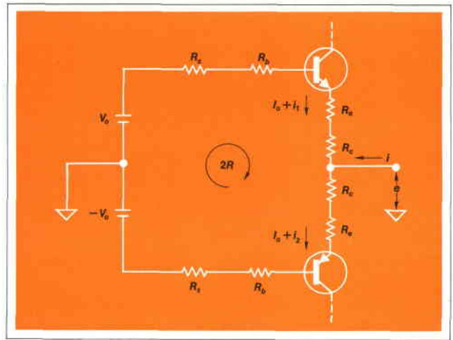
Fig. 5. To find optimum R_e input is grounded, voltage applied to output.
