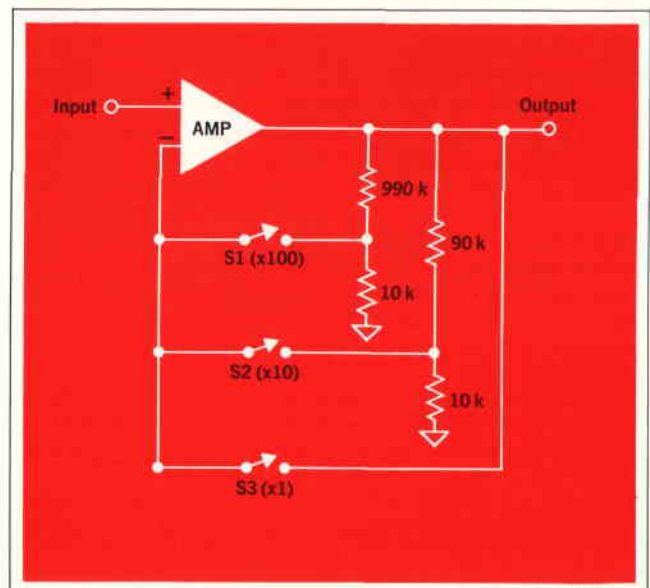
Fig. 12. DC amplifier gain switching.
