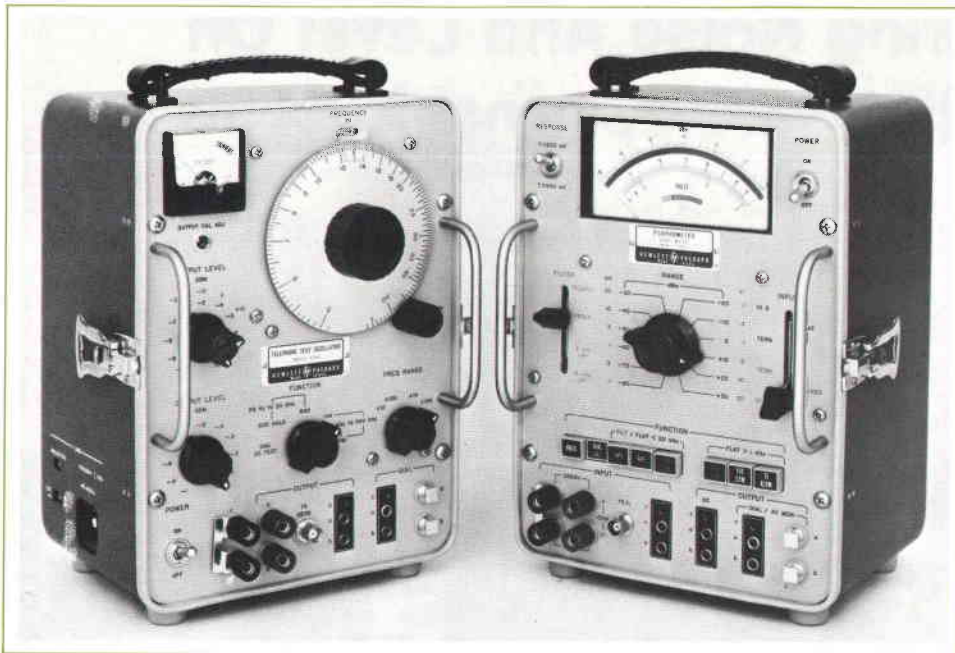
Fig. 1. The HP Model 236A Opt H10 Test Oscillator (left) and the Model 3556A Psophometer are designed specifically for making measurements on telephone systems using CCITT standards (most systems outside the United States and Canada).
