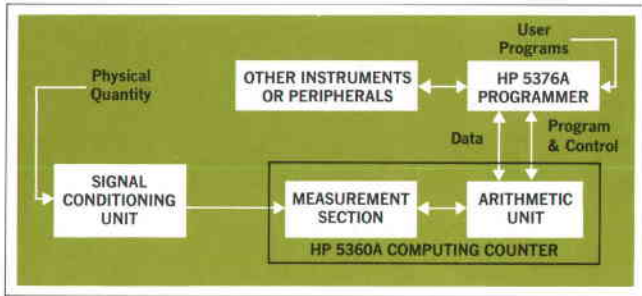
Fig. 1. Computing-counter systems, like computerized systems, can make measurements and arithmetically manipulate the data resulting from the measurements, all under program control. Applications are in data reduction, statistical analysis, process control.
