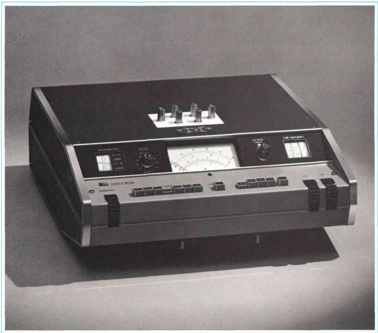
Fig. 2. Pushbutton controls simplify Q measurements with the new HP Model 4342A Q Meter. Q from 5 to 1000 can be measured in a frequency band from 22 kHz to 70 MHz.
