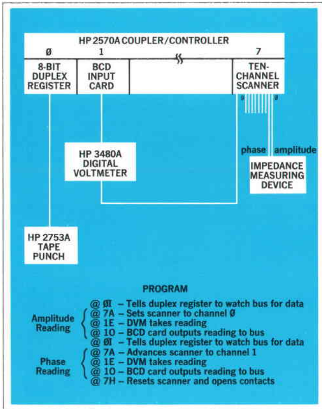
Fig. 6. This system digitizes the analog output of a mechanical-impedance measuring device used in noise-suppression studies. The punched tape is later analyzed by computer.
