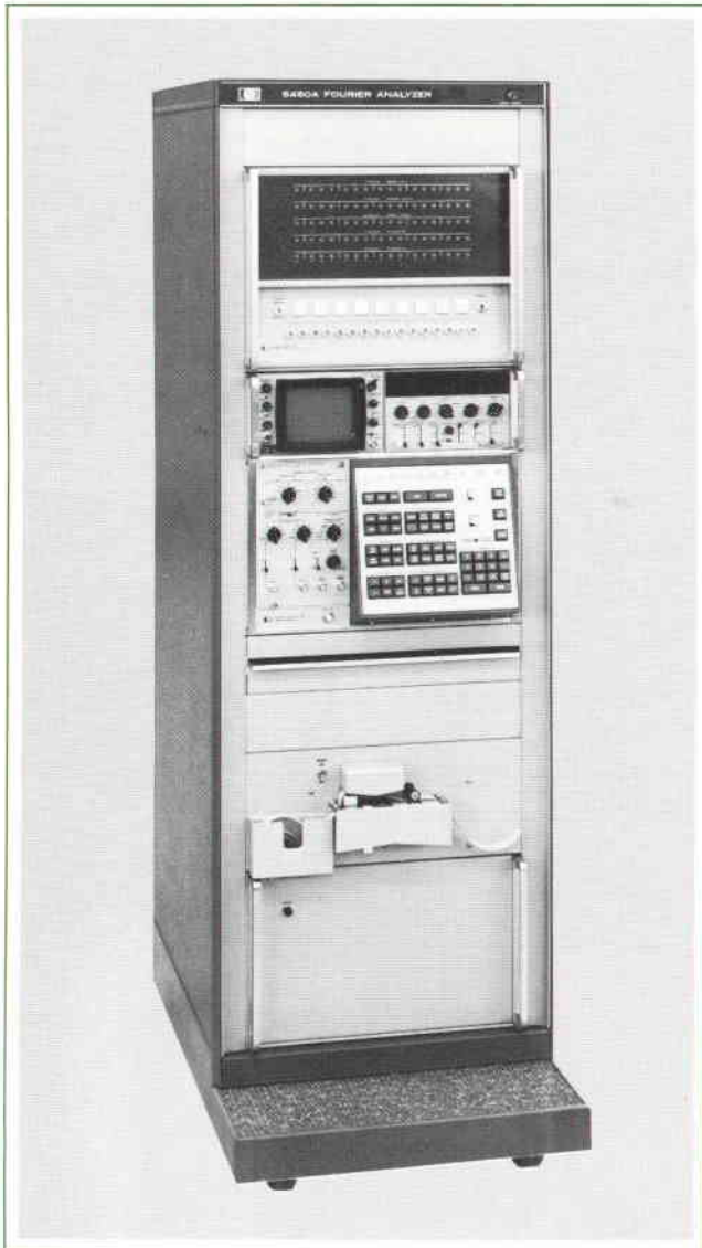
Fig. 1. Model 5450A Fourier Analyzer is a flexible, push-button-controlled, modular, digital instrument, useful for analyzing waveforms and time series in a wide variety of systems and processes. It uses a standard HP computer for memory and computation, but requires no knowledge of computer programming. When it isn't doing Fourier analysis, the computer can be used separately.
