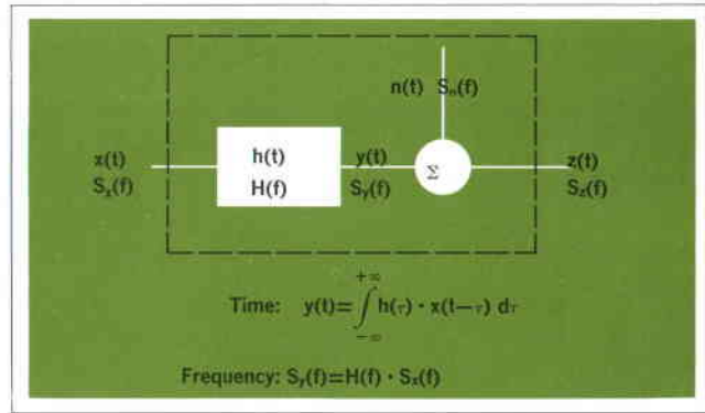
Fig. 3. Is the output z(t) caused entirely by x(t) or is there also unrelated noise n(t) ? What is the form of the relationship between x(t) and y(t) ? The transfer function H(f) provides an answer to the second question. A quantity called the coherence function answers the first.
