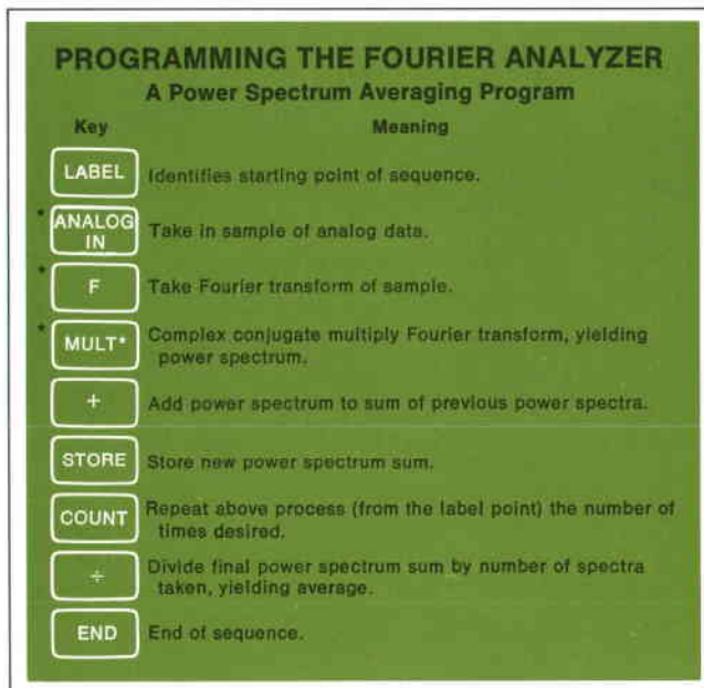
Fig. 8. An often-used routine is the power spectrum averaging program. After the steps are entered into the analyzer's memory, the program can be listed on the teleprinter. Errors can be corrected by adding, deleting, or modifying steps. Another keystroke makes the program execute. Model 5450A will compute one 1024-point spectral estimate (the three steps marked*) in 2.4 seconds or less.
