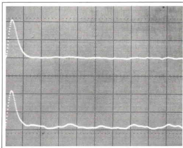
Fig. 6. Crosscorrelation between white noise input and the output of a fourth-order linear system has the shape of the system impulse response. Lower trace is the cross-correlation function computed directly. Upper trace was computed by inverse transforming the system transfer function, which was calculated by dividing the input-to-output cross power spectrum by the input power spectrum. Both traces are the average of 25 measurements. Upper trace is smoother as a result of taking into account the actual input power spectrum.
