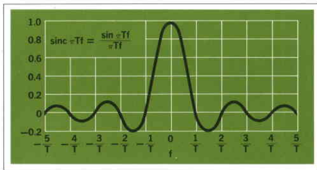
Fig. 7. Spectral lines of a sampled function will have this \sin x/x shape if the function isn't periodic in the record length T . Hanning weighting doubles the width of the main peak, but causes later peaks to fall off at 18dB per octave instead of 6dB per octave.
