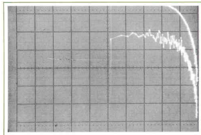
Fig. 5. Transfer function of second-order highly damped system and cross power spectrum of input and output measured by digital analyzer. Spectra of twenty-five sample records were averaged. Not only do the magnitudes of \overline{H} and \overline{G_{yx}} differ, but also the statistical uncertainty in \overline{G_{yx}} is much greater. This is because the computation for \overline{H} takes into account the input power spectrum G_{xx} , whereas the computation for \overline{G_{yx}} does not.
