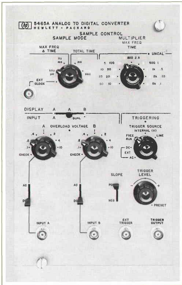
Fig. 3. Analog-to-digital converter is the principal input device for analog signals. It can be operated as a single-channel unit or a dual-channel unit. The maximum sample rate for single-channel operation is 20\mu\text{s} per data point; the minimum rate is one sample in every five seconds. Data can also be read into the analyzer via peripheral devices, such as a tape reader or a teleprinter.
