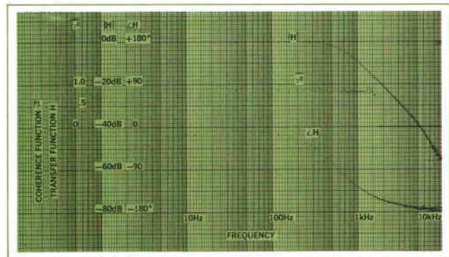
Fig. 4. Transfer function of a second-order highly damped system measured by digital analyzer. Coherence function \overline{\gamma^2} = 0.8 indicates the presence of uncorrelated noise in the system (1.0 would indicate no noise), but transfer function is smooth and well defined, indicating a good measurement in spite of the noise.
