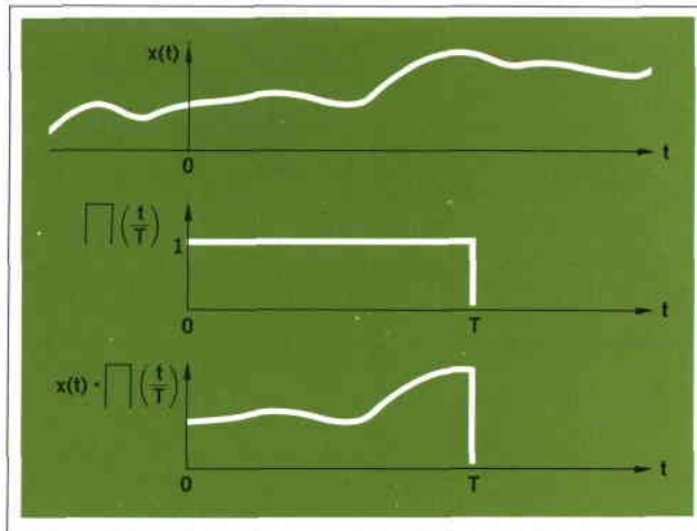
Fig. 6. When a T -second record is taken of an analog input, the effect is to multiply the input by a square window function. If the input isn't periodic with period T , the spectral lines of the input will not be lines but will have the \sin x/x shape shown in Fig. 7. To reduce this effect, Model 5450A Fourier Analyzer has built-in Hanning window-shaping functions.
