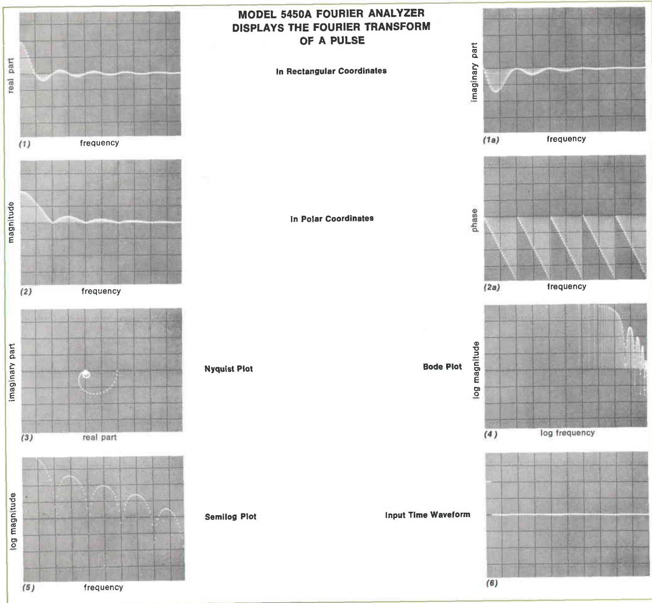
Fig. 5. The analyzer has a display mode to suit every need, and it changes from one to another at the touch of a button or the flick of a switch. In every case the readouts on the display unit and the A-D converter indicate scale factors and type of display.
