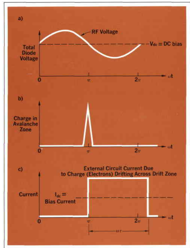
Fig. 5. Charge builds up in avalanche zone just as microwave voltage falls below breakdown level. Movement of charge across drift zone causes rectangular current waveform in external circuit.
