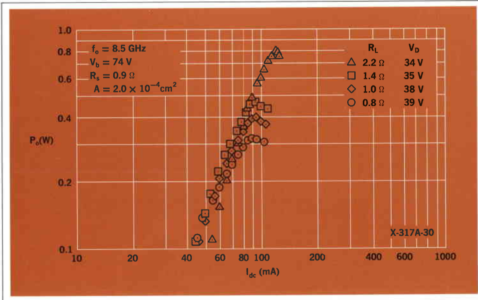
Fig. 9. Typical power output as a function of bias current with load resistance as a parameter. Power limits when V_b = \frac{1}{2} V_{bd} .
