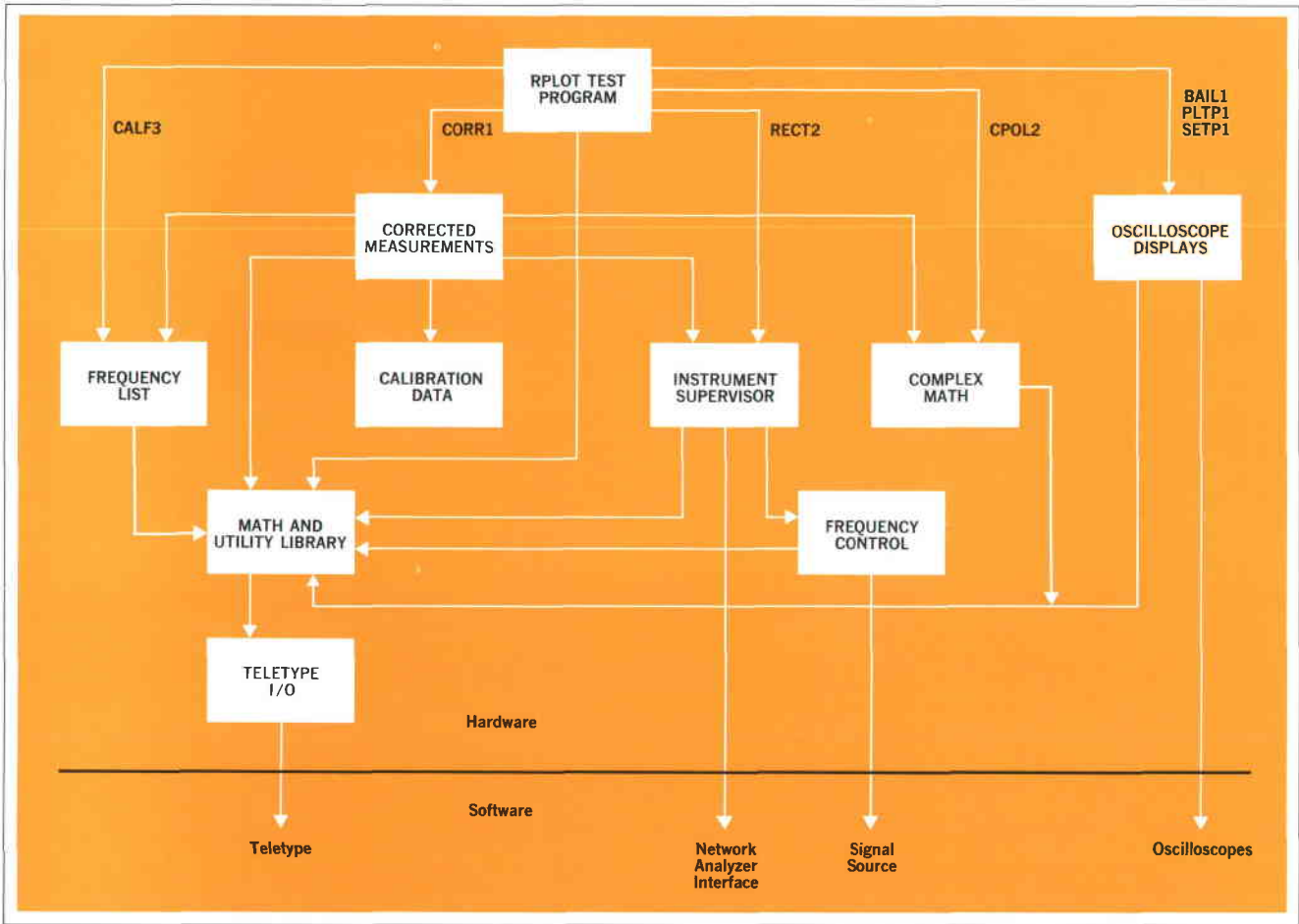
Fig. 4. Hierarchy of routines used by the example FORTRAN program RPL0T of Fig. 3. Here the special test program used only the upper layers, through a few high-level commands. The layered structures, however, can be accessed at any level to suit the application at hand.
