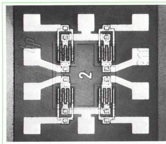
Fig. 1. Typical four-transistor monolithic array. Direct connections between transistor elements are made by metallization pattern.
