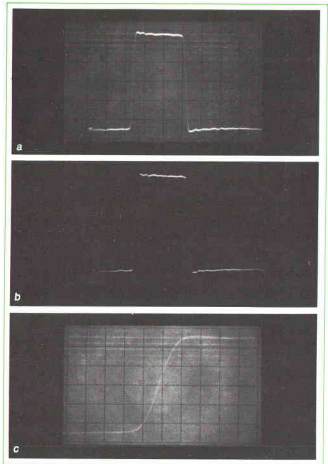
Fig. 3. Automatic film and phosphor 'fogginess' with internal CRT flood gun increases single-shot trace writing rate (A) over that obtained without flood gun (B). Leading and trailing edges of fast pulse ( t_r = 1.5 ns) become visible with flood gun illumination. (Sweep time: 10 ns/cm.) Photo C shows one sweep of same pulse with 1 ns/cm sweep time.
