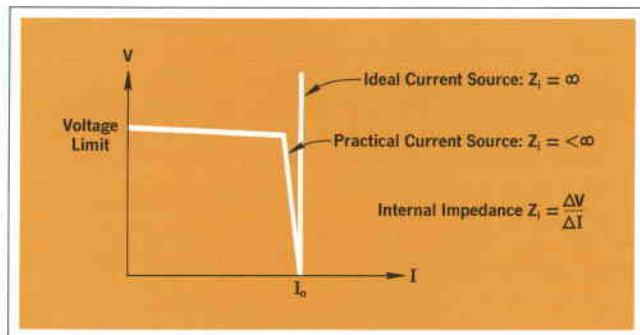
Fig. 1. An ideal current source has infinite internal impedance, delivers the same current, I_0 , to any load, and supplies infinite voltage to an open circuit. A practical current source has a Z_i which is finite, but as high as possible. It should also have an adjustable voltage limit to keep the load from being damaged.
