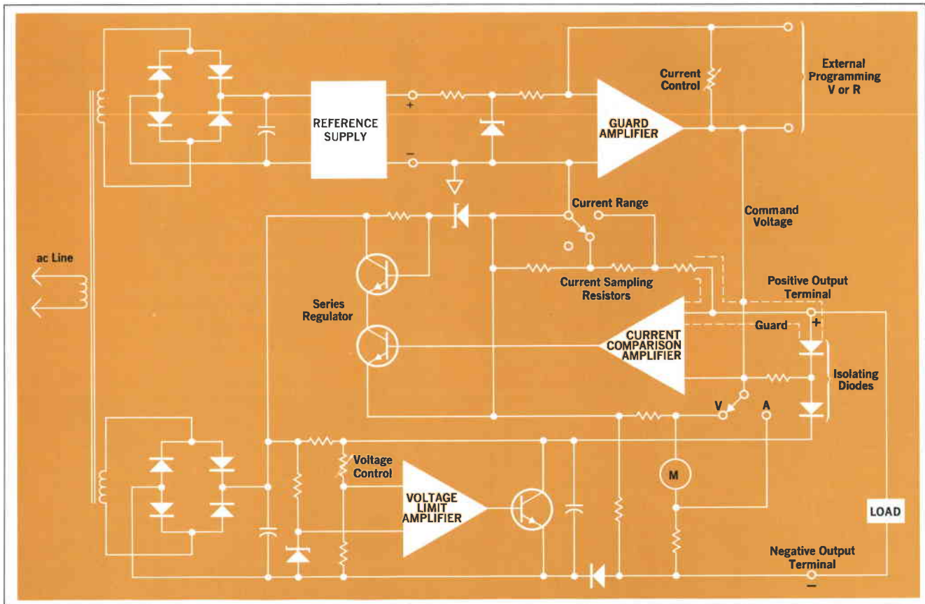
Fig. 4. Command voltage for current regulator comes from internal reference supply or from external programming voltage or resistance. Voltage-limit circuit quickly draws current away from load when load voltage exceeds voltage limits and isolating diodes turn on. High-gain regulator and absence of reactive elements in output give high output impedance, fast programming, and freedom from current overshoots.
