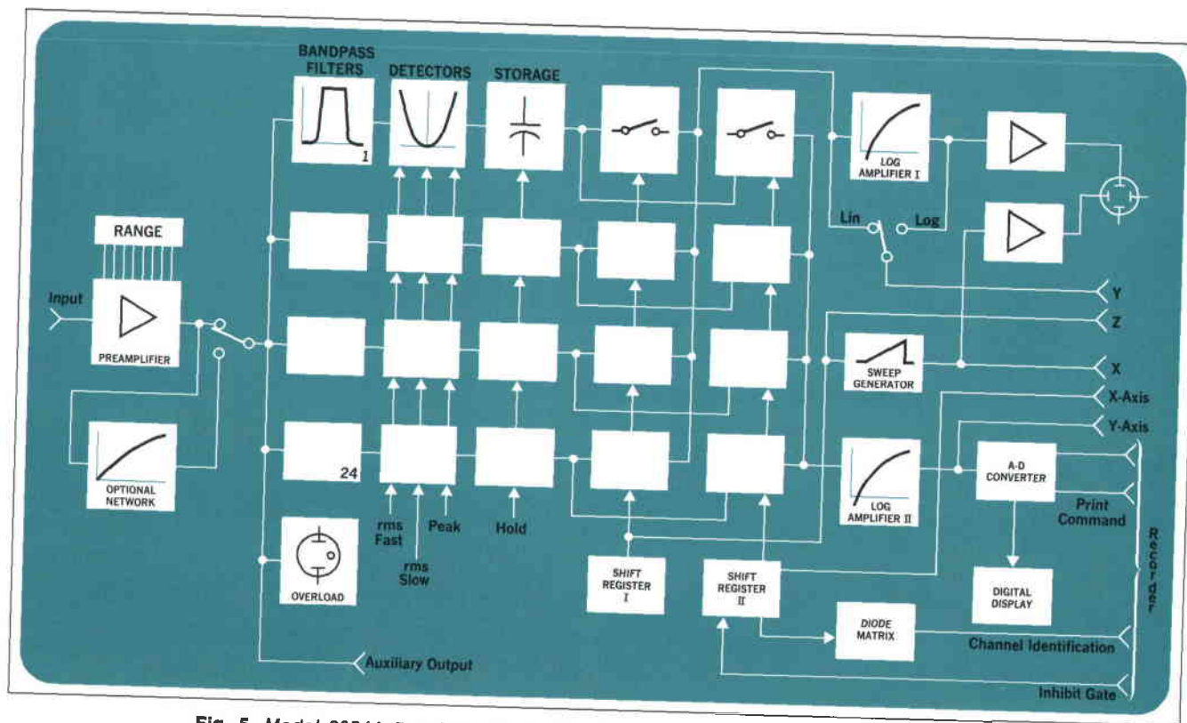
Fig. 5. Model 8054A Real-Time Audio Spectrum Analyzer has rms detectors with time constants of 0.1 and 1 second; they can measure signals which have crest factors up to 5. The 'hold' mode freezes the display, and the 'peak' mode captures and holds the peak values of single-shot transients.
