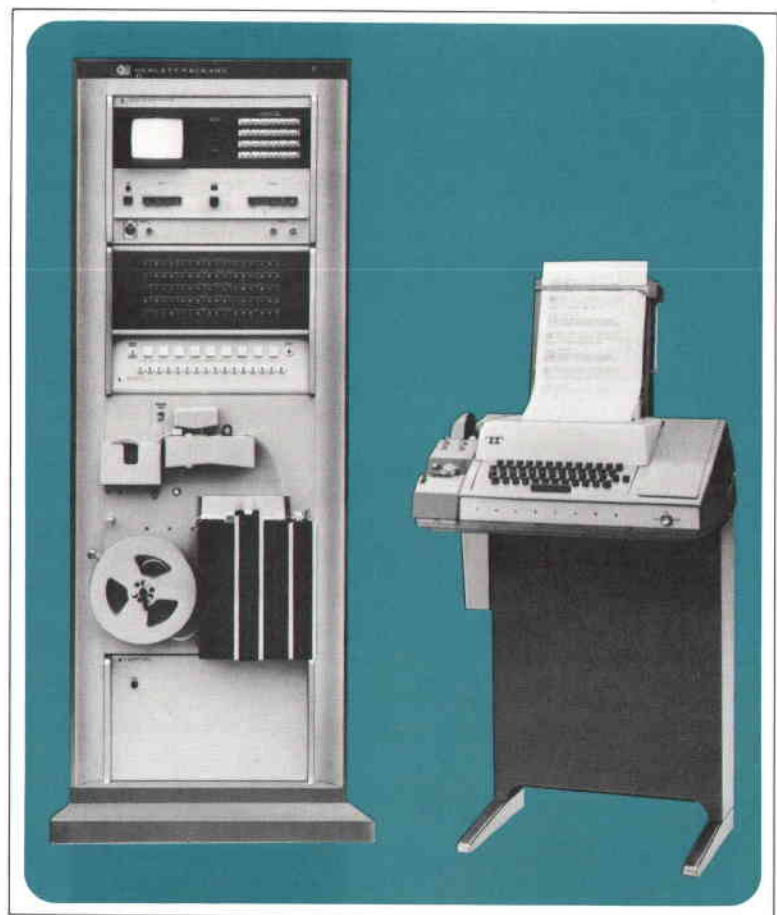
Fig. 1. Model 80501A Audio Data Processor consists of a real-time audio spectrum analyzer (with CRT) which measures the frequency spectra of audio-frequency inputs, a digital computer which processes the measured spectra, and peripheral devices. A typical application is aircraft noise analysis and evaluation. Real-time processing gives results almost immediately so appropriate action can be taken if required.
