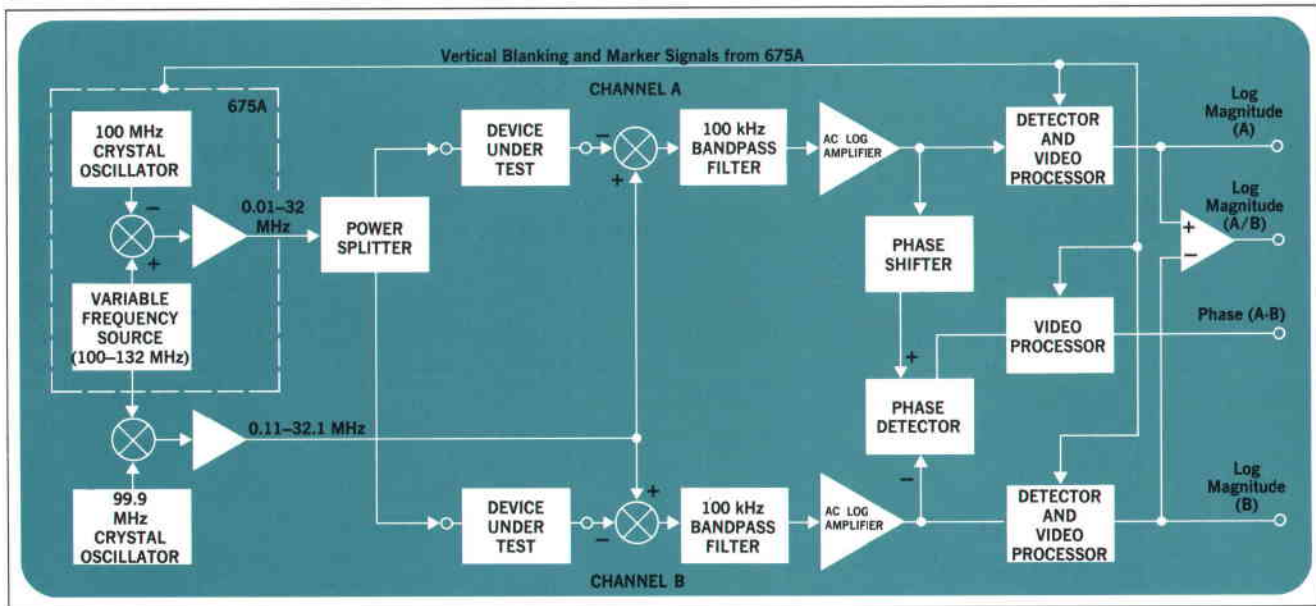
Fig. 2. The RF output of the Model 675A Sweeping Signal Generator is connected to the RF input terminal of the Model 676A Tracking Detector. Phase shift in both channels is equal so that any variation introduced in one channel will appear at the PHASE A-B output.
