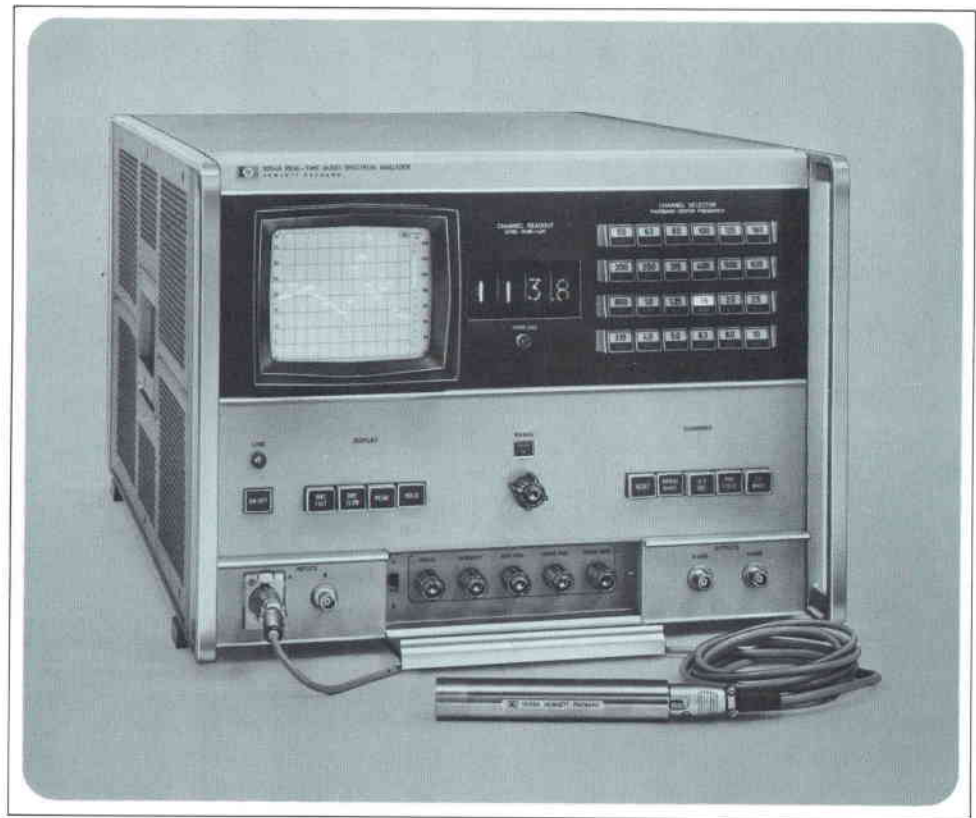
Fig. 3. Model 8054A Real-Time Audio Spectrum Analyzer divides the audio spectrum into 24 third-octave frequency bands and measures the rms or peak value of the signal in each band. Results are displayed on the CRT. Single bands can be selected for digital readout.
