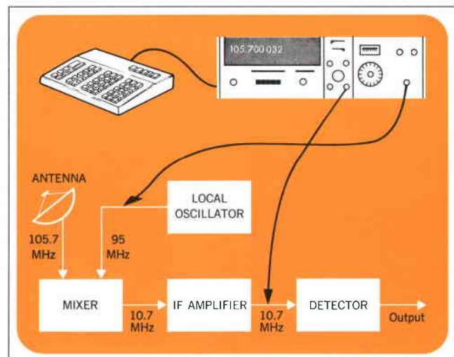
Fig. 6. This is an example of how the keyboard and the computing counter can work together to make measurements that would be awkward for conventional counters. The received signal at 105.7 MHz is too weak to be counted. A simple six-step program directs the counter to measure the 95 MHz LO frequency and the 10.7 MHz IF and add them to get the received frequency.
