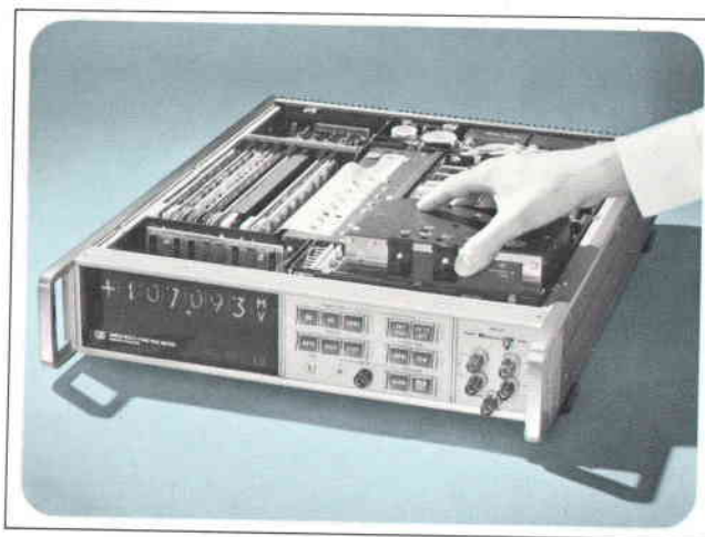
Fig. 12. True rms ac-dc converter is installed in the HP Model 3450A as a plug-in.
