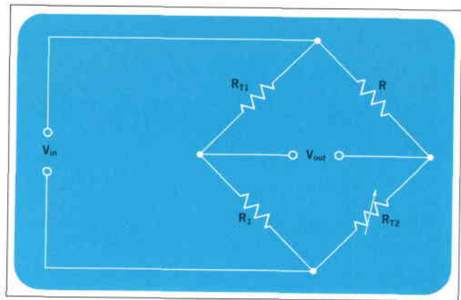
Fig. 9. A four-terminal ratio measurement is required on this balanced bridge network to make V_{out} independent of any \Delta V_{in} .
