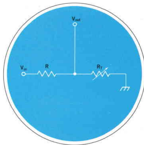
Fig. 8. To accurately determine the value of R_T , the ratio of V_{out} to V_{in} is more important than the absolute value of V_{out} . Accuracy is then independent of variations in V_{in} .
