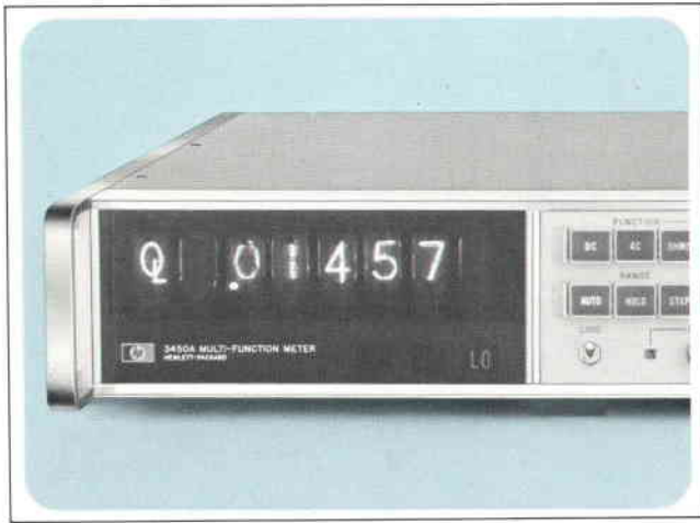
Fig. 11. Indication shows ratio underload on the HP Model 3450A when reference voltage drops below a usable level.
