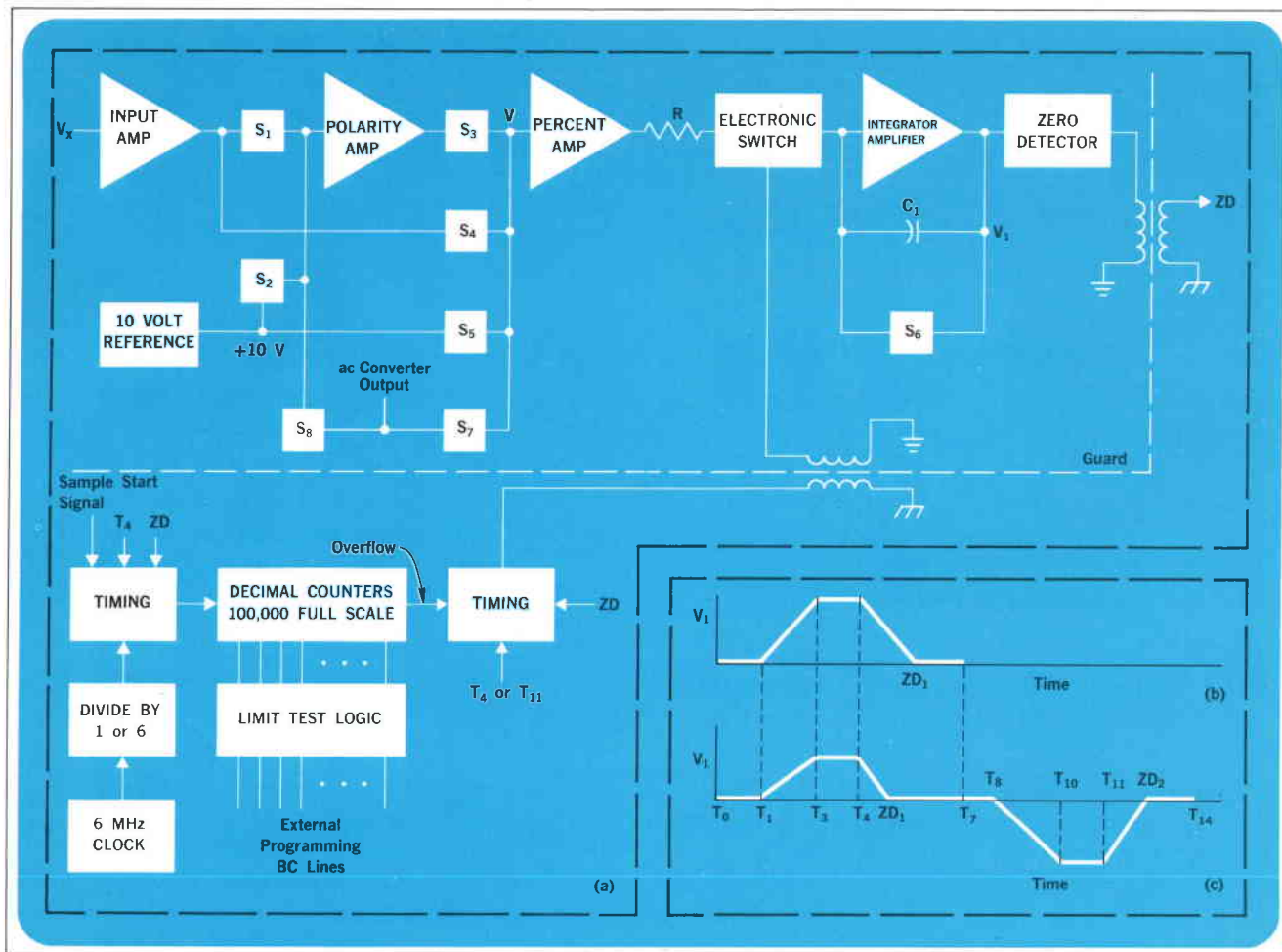
Fig. 7. In addition to the basic blocks of Fig. 5, the HP Model 3450A includes the signal processing input amplifier and a limit test logic section (a). Voltage waveforms on the integrating capacitor C_1 for dc measurements (b) and dc ratio measurements (c).
