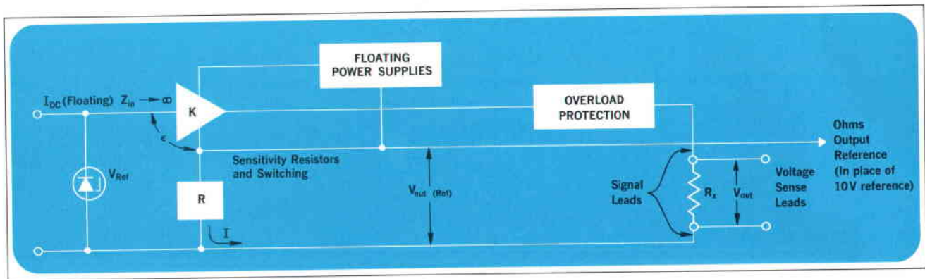
Fig. 14. Ohms measurements are made by taking the ratio of V_{out} to V_{out(Ref)} . Resistor R determines current I which also flows through R_x . Thus the ratio of the two voltages is the ratio of R_x to R . Amplifier error \epsilon and the magnitude of V_{Ref} do not affect measurement accuracy.
