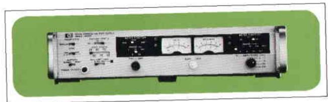
Fig. 3. Model 8717A Transistor Bias Supply has slide switches for rapid selection of bias conditions. The transistor being biased is an integral part of a feedback system in the supply which maintains the accuracy and stability of the bias conditions.
