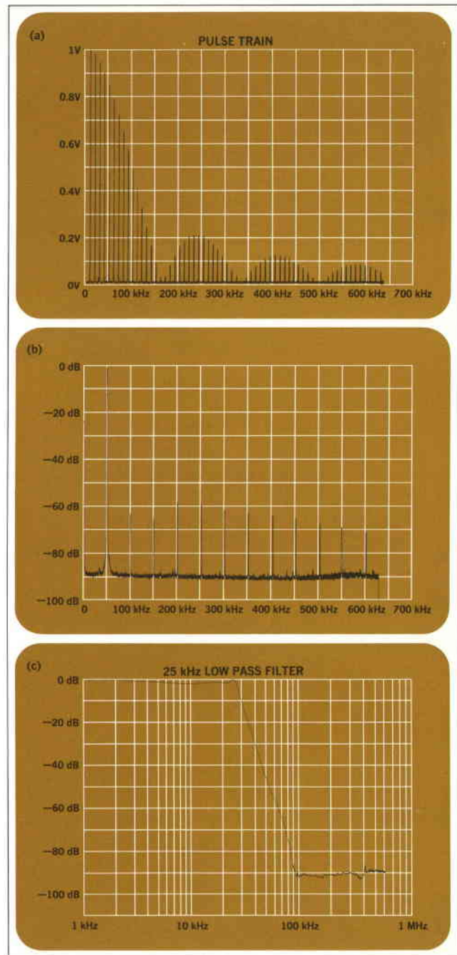
Fig. 1. The frequency spectrum of a pulse train plotted on linear axes (A) clearly show the \sin x/x envelope of the fundamental and harmonics. Harmonic components of a 50 kHz sine wave (B) are displayed very clearly on a logarithmic amplitude scale and a linear frequency scale. Plotting the frequency response of a filter on two logarithmic axes (C) gives good resolution at both extremes of amplitude and frequency.
