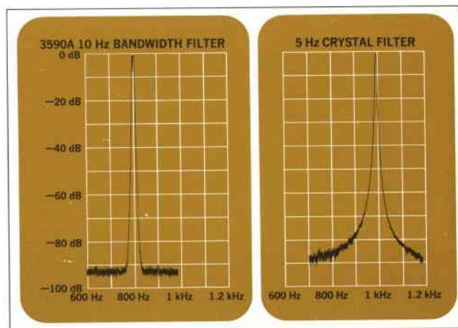
Fig. 5. Comparison of the 10 Hz active bandpass filter in the Model 3590A with a typical crystal filter also designed for wave analysis. While the crystal filter has a narrower bandpass at the 3 dB points, it is broader below 30 dB. The 10 Hz active filter offers more selectivity when measuring small signals adjacent to large signals.
