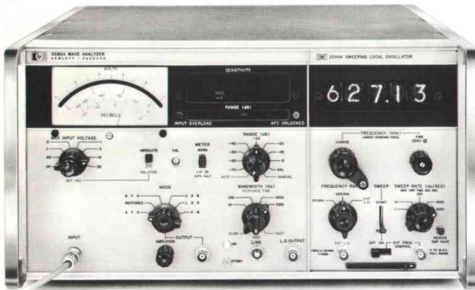
Fig. 2. This new HP Model 3590A Wave Analyzer makes selective measurements from 20 Hz to 620 kHz over an 85 dB dynamic amplitude range. Automatic amplitude ranging, internal electronic sweep, lighted meter scales and both log and linear X-Y recorder outputs are included.
