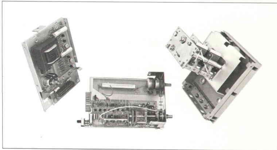
Fig. 3. By molding a number of parts as part of the front panel (right) assembly time is reduced while increasing precision of positioning of a number of parts. The printed circuit board assembly (center) plugs into the front panel. Power supplies (left) plug into the main board. Standard \frac{1}{3} module side frames lock the assemblies together.
