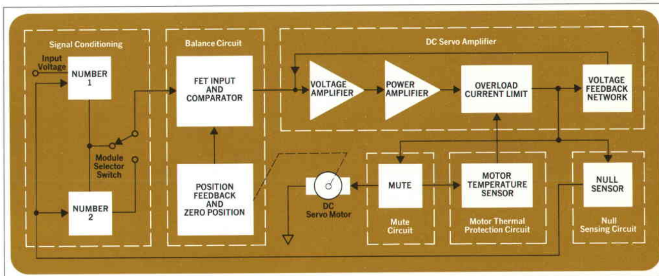
Fig. 4. Six functional blocks make up the Model 7004A main frame. Numbers 1 and 2 in the Signal Conditioning area are spaces for the plug-ins.
