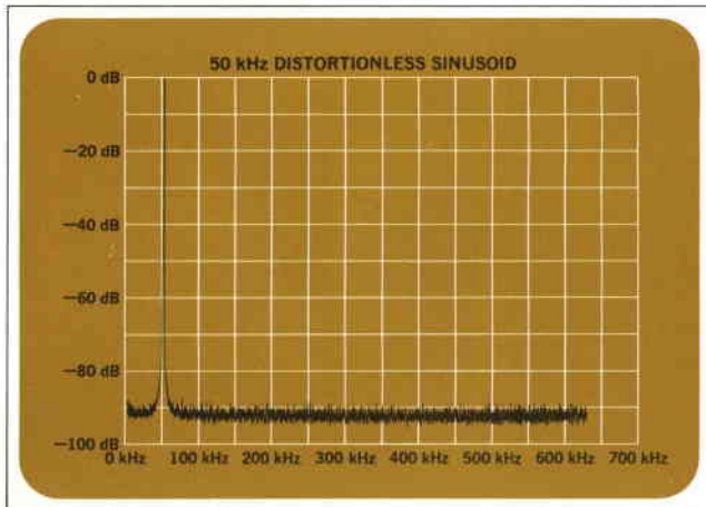
Fig. 3. Measuring a pure 50 kHz sinusoid demonstrates that the Model 3590A typically contributes no spurious or distortion products to the frequency spectrum.
