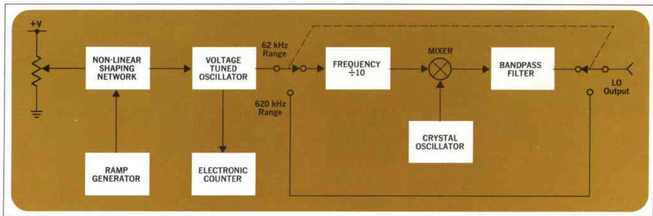
Fig. 4. Tuning circuitry in the Model 3594A Local Oscillator plug-in may be set to cover either a 620 kHz or 62 kHz range. The narrow range offers better accuracy, stability and resolution for those applications not needing the wide range.
