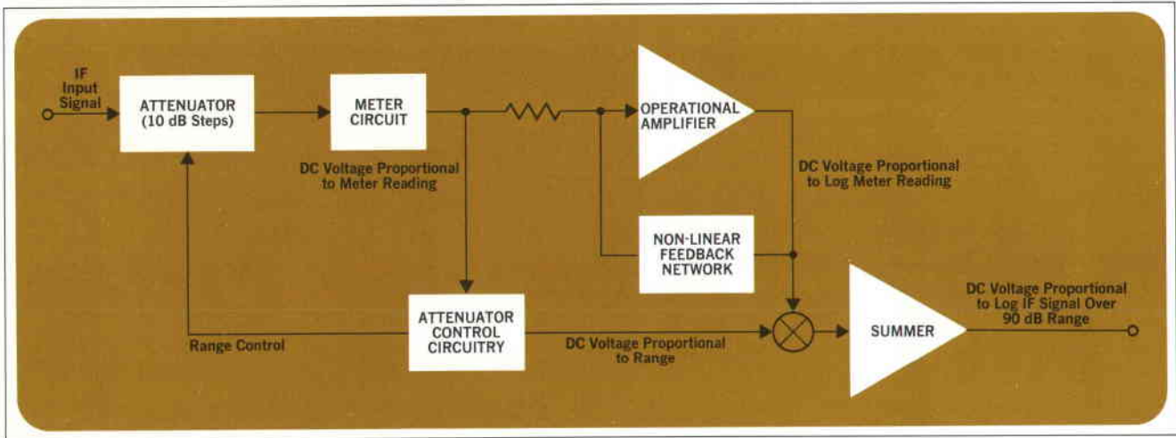
Fig. 6. Metering circuit and logarithmic amplifier. The IF attenuator is set automatically to the proper range. Two dc levels—one proportional to range setting, the other logarithmically proportional to the metered signal—are summed to give an output level logarithmically proportional to the IF signal amplitude, calibrated in volts per dB over a 90 dB display range.
