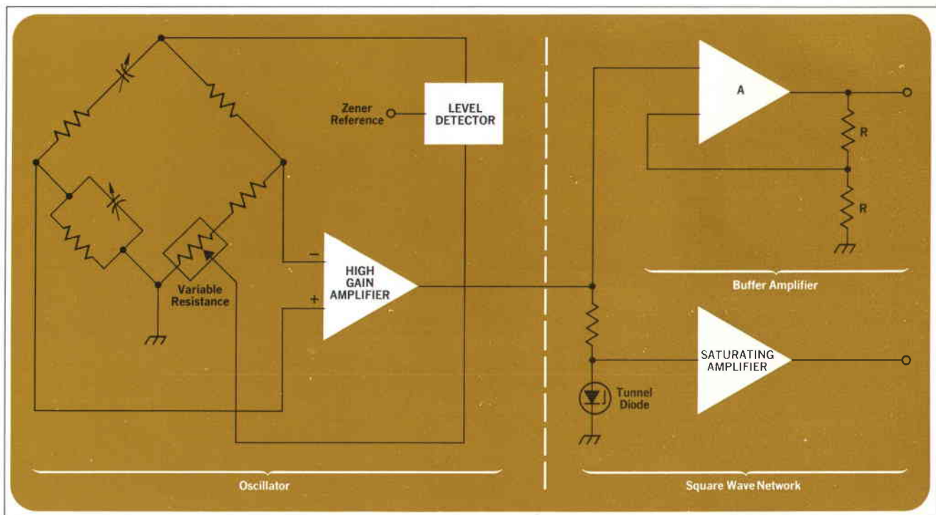
Fig. 2. A Wien bridge (left) is the heart of the two oscillators. Additional circuitry at the right amplifies the sine wave and also provides the square wave output of the Model 209A.
