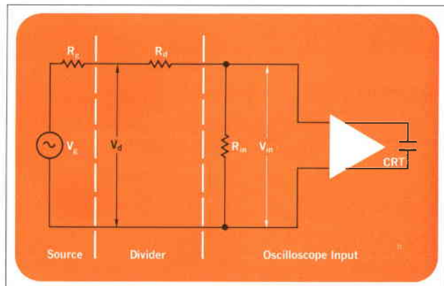
Fig. 3. Division ratio in a typical resistive divider probe is determined by R_d , R_3 and R_{in} .
