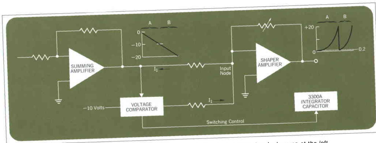
Fig. 6. The two exponential curves at the right are generated from the single ramp at the left. As the ramp voltage goes from 0 to -10 , current is drawn from the shaper amplifier causing its output to rise exponentially from 0.2 to 20 volts. At -10 volts on the ramp, the voltage comparator switches the precise amount of current being drawn. This causes the shaper amplifier to reset to 0.2 volt. The voltage comparator continues to supply current as the ramp proceeds from -10 to -20 volts, resulting in the second exponential B, at the right.
