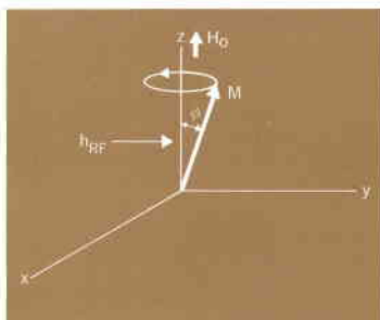
(d) Precession of the net magnetization vector due to RF magnetic excitation.
