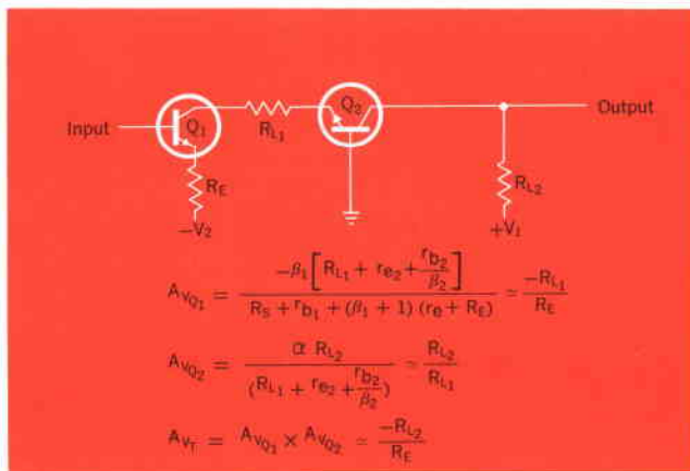
Fig. 3. Transistorized equivalent of the cascode amplifier. A_{VQ_1} and A_{VQ_2} are the voltage gains of transistors Q_1 and Q_2 ; A_{VT} is the total amplifier gain; \beta_1 and \beta_2 are the beta current gains of the transistors, r_e and r_b are resistances of the emitter and base respectively; R_s is the source resistance of the generator driving the amplifier.
