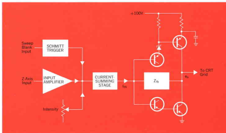
Fig. 2. The Model 1300A z-axis amplifier is direct coupled. I_{\Sigma} is the sum of currents from three sources, shown.
