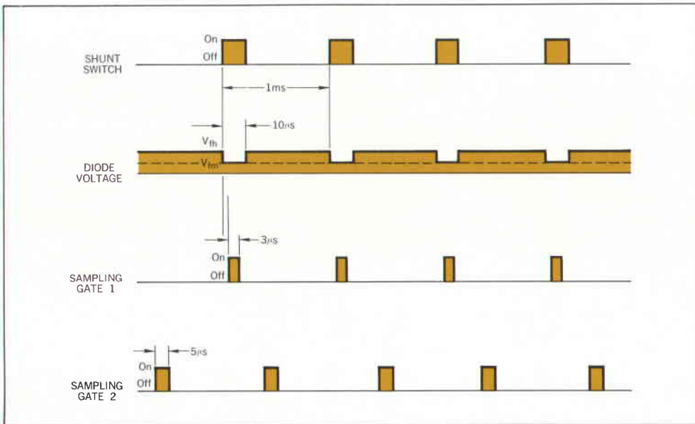
Fig. 8. Timing diagram of the thermal resistance measurement. Sampling Gate #1 samples V_{tm} and it can be delayed as long as 6 \mu s from the turn-on time of the shunt switch. This delay permits diodes with a long minority carrier lifetime adequate time to reach V_{tm} from V_{th} . Sampling Gate #2 samples V_{th} .
