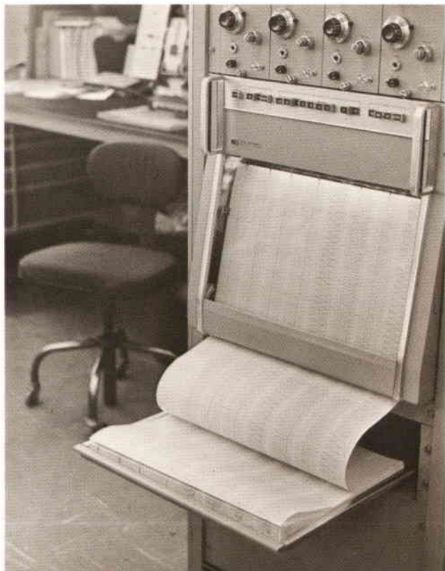
Fig. 2. Unlike most pressurized ink recorders, the new recorder can use Z-fold chart paper, which is much more convenient than rolled paper because it allows any part of a record to be examined easily, even while recording.
