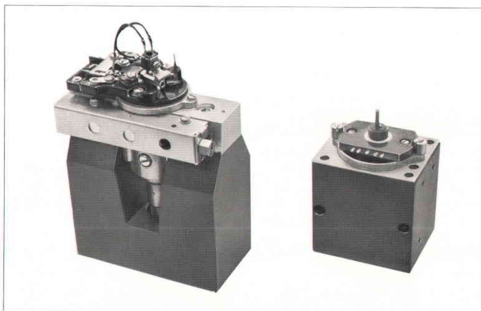
Fig. 10. New pen motor (r), is lighter and smaller than older type (l), and has smaller stray external magnetic field.
