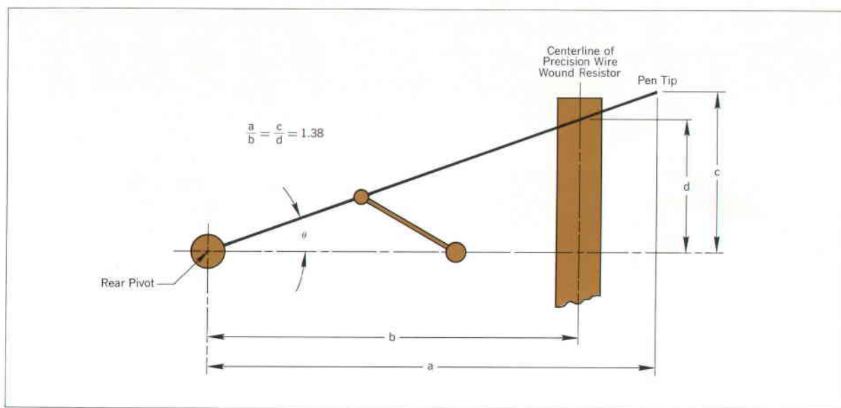
Fig. 7. Transducer near pen tip is linear. Ratio of tip motion to pickoff-wire displacement is 1.38 to 1.
