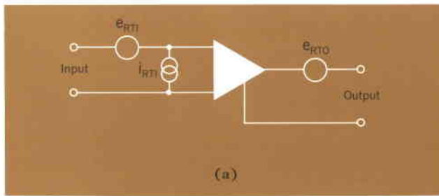
Fig. 2. Offset voltage and offset current (a), both referred-to-input because they are gain-dependent, and the voltage referred-to-output which is not gain-dependent, are the major parameters in determining total offset. Insufficient common-mode-rejection is another source of offset error (b). The common mode signal at the output is equal to e_{CM} \left( \frac{\text{Gain}}{\text{CMR}} \right) .
