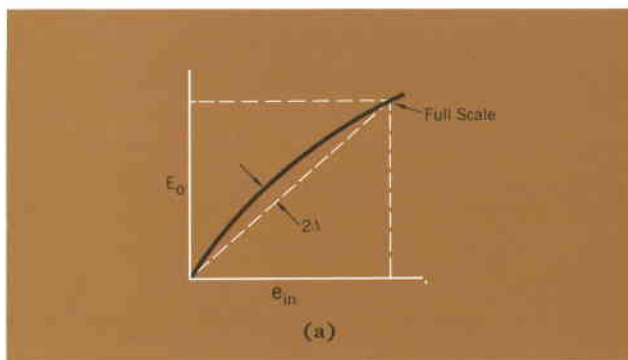
Fig. 3. Comparing the 'terminal linearity' method of specifying gain accuracy (a) with the 'best straight line' method (b) shows that while the 'best straight line' method results in better numbers on specifications, the 'terminal linearity' method results in a more accurate statement of real usefulness.
