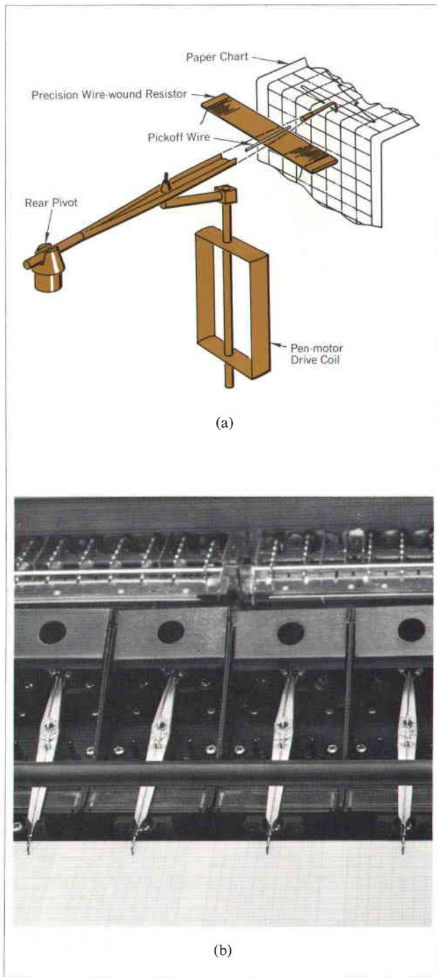
Fig. 6 (a). Pen drive mechanism is simple, yet very linear. As pen motor rotates, pen tip describes a line that is straight within 0.005" across 4 cm channel. Position-sensing transducer is located near pen tip to detect linkage errors. Pickoff wire does not touch wirewound resistor, so transducer wear is not a problem. (b). Transducer resistors can be seen just below transverse rod in photograph.
