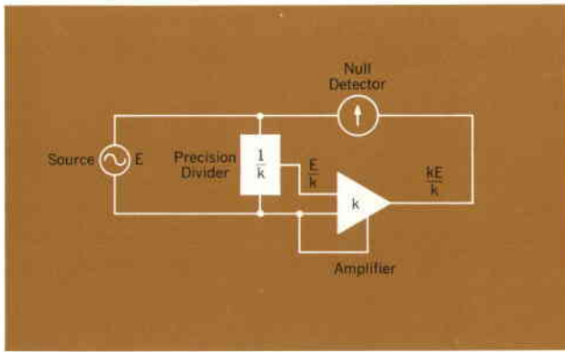
Fig. 4. Use of the bridge method of checking gain linearity of an amplifier with gain K is relatively inexpensive and rapid. Precision depends mainly upon the accuracy of the voltage divider and the sensitivity of the null detector.
