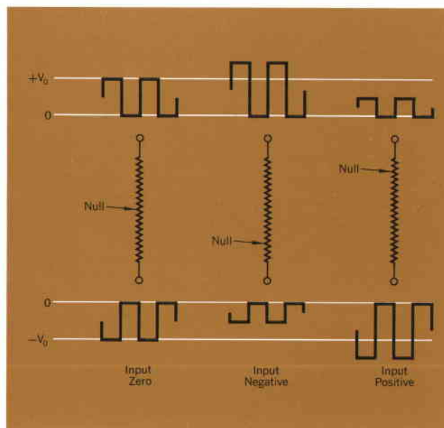
Fig. 8. 20 kHz square waves, 180° out of phase, are applied to ends of transducer resistor, creating a null which is shifted as a function of the input signal. Servo system senses pen position relative to the null and drives pen to follow null.
