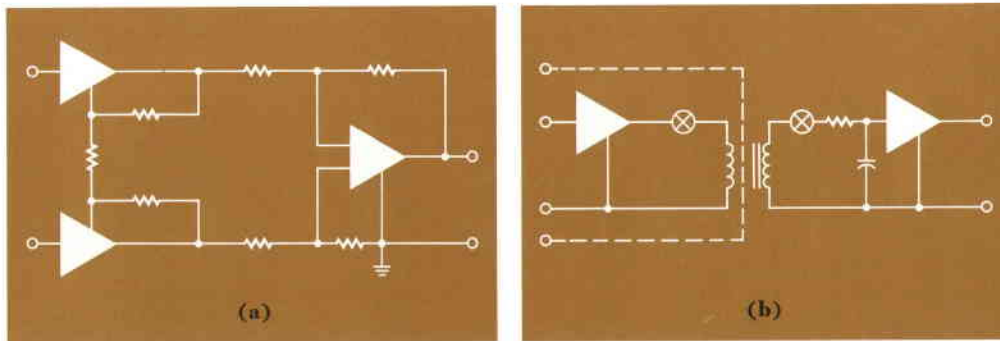
Fig. 1. Two common configurations of data amplifiers are the direct-coupled differential (a) and the carrier-coupled design (b).
