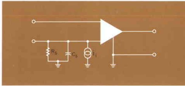
Fig. 4. Sources of additional offset error are due to injected current, i_i , source resistance and capacitance.
