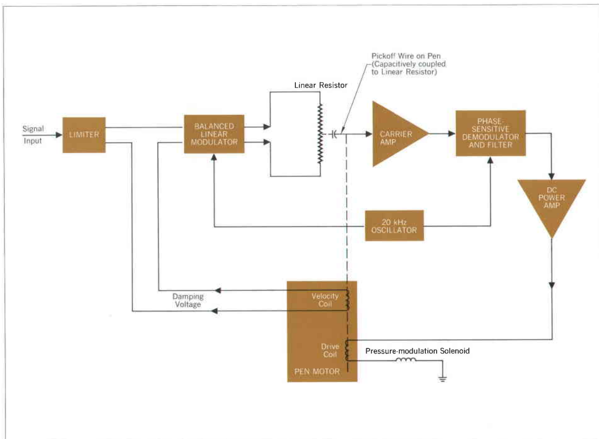
Fig. 9. Electrical drive circuit for one channel of ink recorder.
