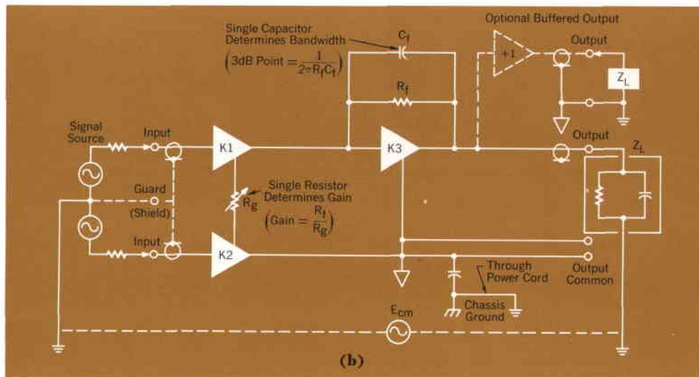
Fig. 2. The new HP Model 2470A Data Amplifier (a) is a differential design consisting of three amplifiers, K1, K2 and K3 (b). Amplifiers K1 and K2 are identical. Power supplies for the three amplifiers are completely isolated from each other to preserve the common mode rejection offered by the design.
