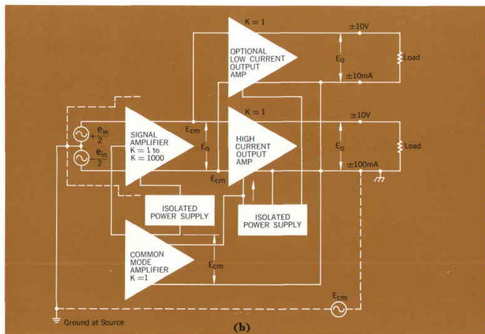
Fig. 3. The HP Model 8875A Data Amplifier (a) uses a common mode amplifier (b) to provide good common mode rejection without the use of a specially shielded power transformer.
