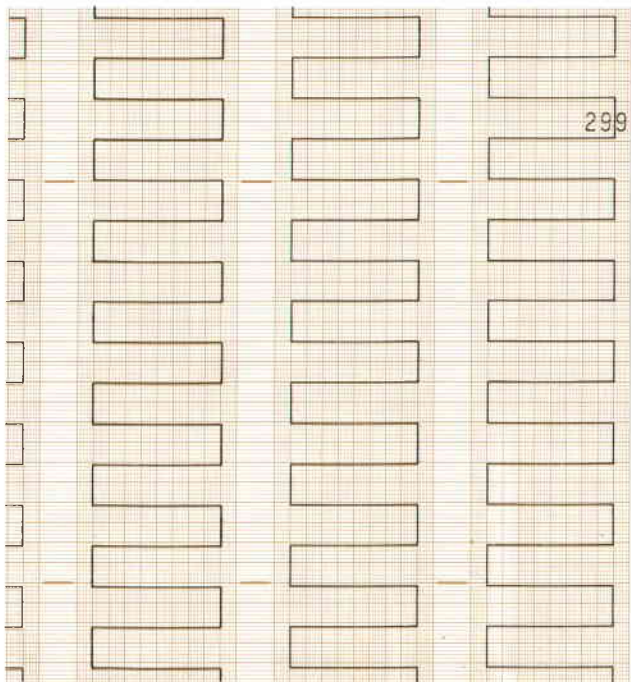
Fig. 4. Chart paper used for ink recording has eight channels, each 4 cm wide with 50 divisions. Recorded square wave shows how ink-pressure modulation prevents loss of trace for step-function inputs.
