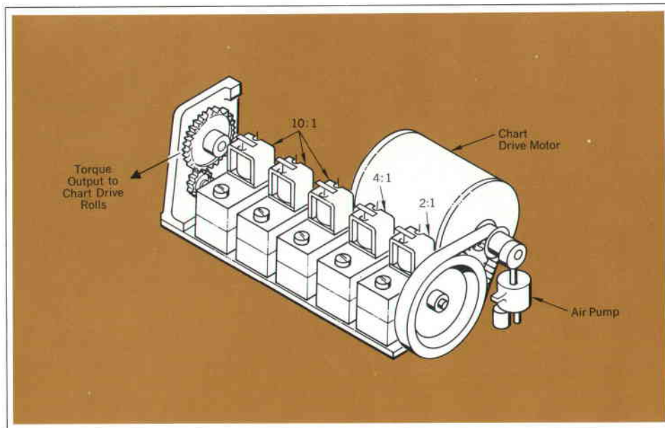
Fig. 11. Simplified chart drive mechanism gives 14 chart speeds with relatively few parts, many of them interchangeable. Different speeds are obtained by switching solenoids to engage or disengage the five reduction gears in different combinations.
