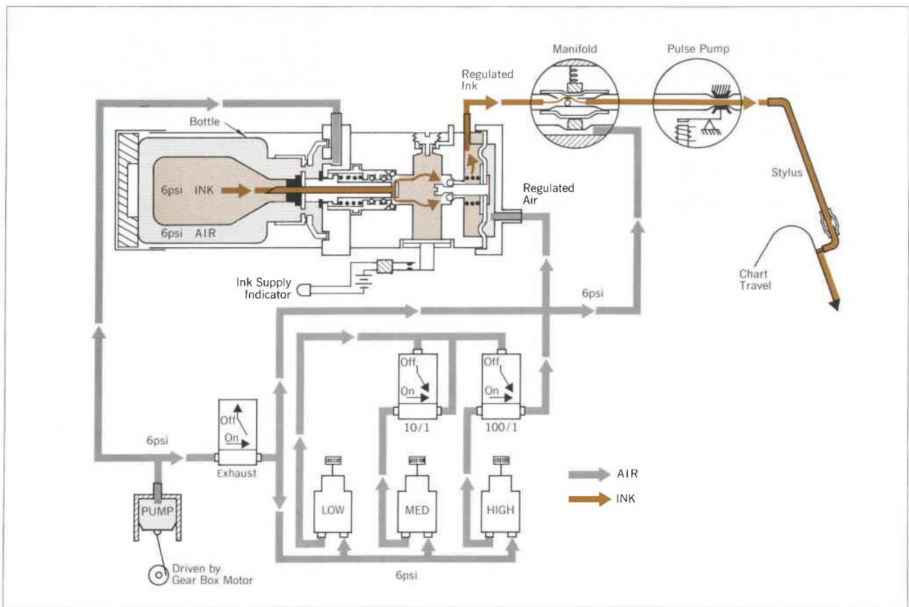
Fig. 5. Diagram of the pressure-modulated ink supply system. One pen is shown, although the manifold supplies all eight.
