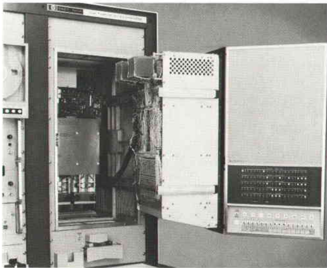
Fig. 5. All elements of hp-2116A Computer are accessible from front of cabinet. Memory modules (the two cube-shaped objects protruding from top of backplane) can be changed in five minutes. Computer is fully enclosed for bench use, weighs only 230 lbs. (10.4 kg) and stands 31½ inches high (782.4 mm). It can be rack mounted.
