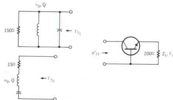
Fig. 12. Transistor oscillator is designed by choosing tank circuit such that \Gamma_s s'_{11} = 1 .
