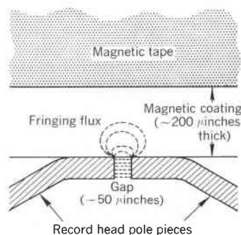
Cross-section of the record process. The iringing flux penetrates the coating and, as the tape moves across the gap, leaves a series of magnetized segments representing the recorded signal.
