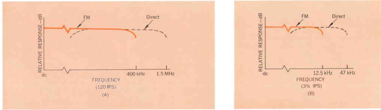
Fig. 2. Frequency response in the FM mode and Direct mode at a tape speed of 120 ips (a) and 3 \frac{3}{4} ips (b). In the FM mode, bandwidth is exchanged for dc response and freedom from dropouts.
