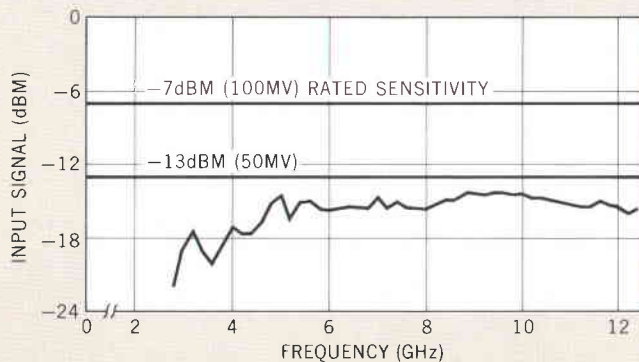
Fig. 2. This sensitivity plot shows the input signal level that is required for counting, that is, to put the panel meter into the green region.
