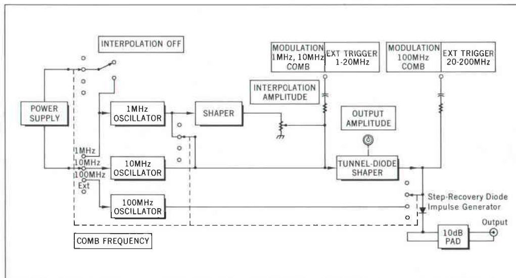
Fig. 7. Block diagram of Frequency Comb Generator. Step recovery diode working into shorted stub line differentiator generates output impulse. One of three crystal oscillators energized by front panel push buttons drives step recovery diode. Tunnel-diode shaper speeds up rise times of lower frequency drive signals sufficiently to drive step recovery diode. 10-dB pad makes output impedance a nominal 50 ohms because of low impedance of shorted stub.
