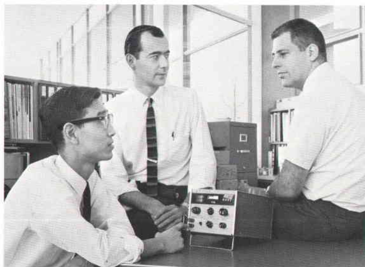
Project leader Katsumi Yoshimoto discusses design of production model instrument with Gregory Justice (center) and Edward Heinsen (right) who developed initial concept of semiautomatic bridge at -hp- Advanced R and D Laboratories in Palo Alto.
