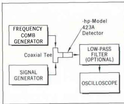
Fig. 8. When Frequency Comb Generator is used for calibration of signal generators, crystal detector acts as mixer to provide sum and difference products between signal generator output frequency and comb frequencies. Oscilloscope serves as zero-beat indicator to show when signal generator output and comb component are at same frequency.
