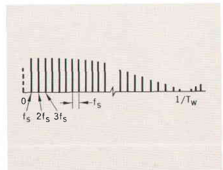
Fig. 6. Frequency domain representation of pulse train shown in Fig. 5. With ideal pulses, frequency components would be of near identical amplitude out to 1/\pi T_w and may go through a null at a frequency of 1/T_w .
