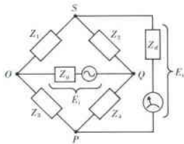
At balance ( E_o = 0 ), Z_1 Z_4 = Z_2 Z_3
