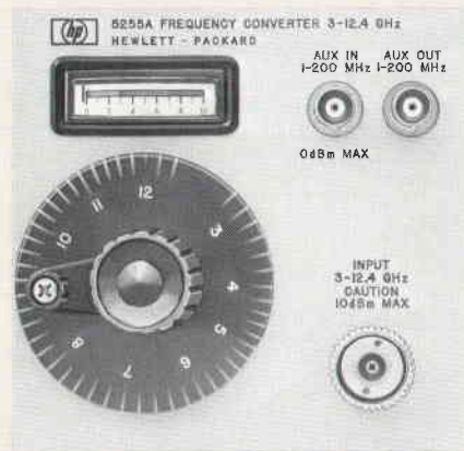
Fig. 1. The dial markings on the cavity tuning dial of the hp Model 5255A Frequency Converter Plug-in are transparent and give a red indication when the cavity is tuned to a harmonic of 200 MHz.
