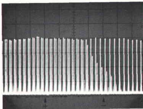
Fig. 9. Frequency response measurement of -hp- Model 360A 700-MHz low-pass filter using Frequency Comb Generator output as stimulus and spectrum analyzer to display results. Input and output combs are shown, displaced slightly with respect to each other for clarity. Comb which extends evenly towards right of display is input comb. Output of filter is comb that drops off in amplitude to right of center. Center screen is 700 MHz, spectrum width is 30 MHz/cm, and vertical calibration is 10 dB/cm, showing filter cutoff slope of approximately 42 dB/100 MHz.
