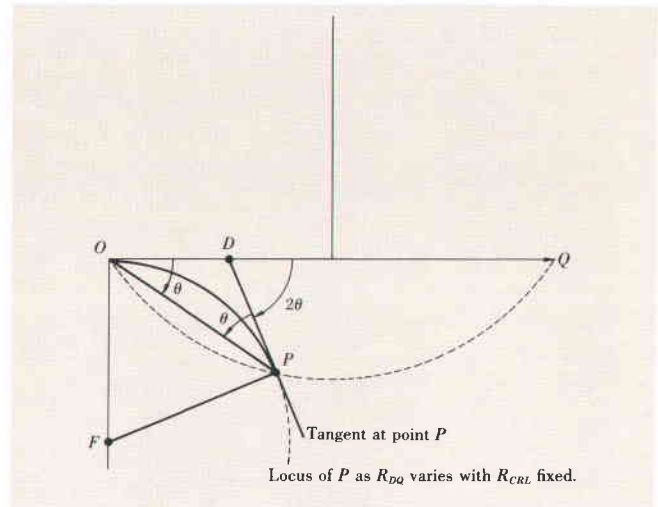
Fig. 4. Determination of phase reference for sensing change in output voltage caused by change in R_{DQ} . Small change in R_{DQ} moves P along path approximating tangent to circular locus of P . Tangent intersects reference vector \overline{OQ} at an angle 2\theta that is twice angle \theta made by vector \overline{OP} with respect to \overline{OQ} .
