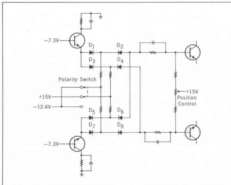
Fig. 6. Polarity of the input to the vertical amplifiers is switched by switching diode gates. In the 'up' or + position, diodes D_1 , D_2 , D_7 and D_8 are turned on while D_3 , D_4 , D_5 and D_6 are reversed biased. The signal path is across D_1 , D_2 , and D_7 , D_8 . Reversing polarity reverses the bias.
