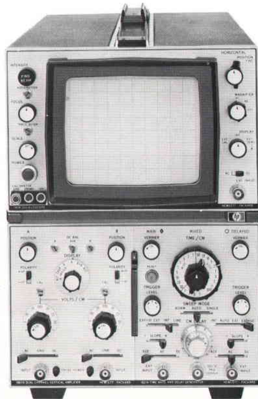
Fig. 3. The front panel of the oscilloscope, shown here \frac{2}{3} actual size, is slightly shorter than this page height and slightly narrower than this page width. Controls are clearly marked and arranged so they are not obscured by cables. Plug-ins are in the lower half of this cabinet version, with CRT beam controls and horizontal amplifier controls in the upper half.
