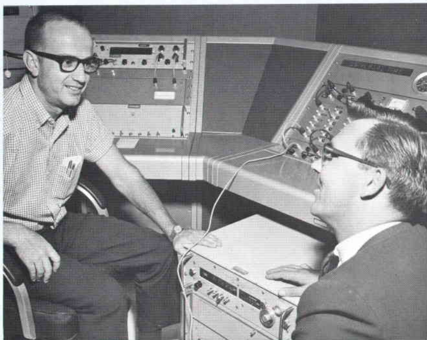
Flying clock (below counter) is compared to NBS frequency and time scales in "clock room" at Boulder Laboratories of National Bureau of Standards. Dr. James Barnes (left), Chief of Atomic Frequency and Time Standards at NBS, and -hp- engineer Lee Bodily discuss techniques of time measurement.
