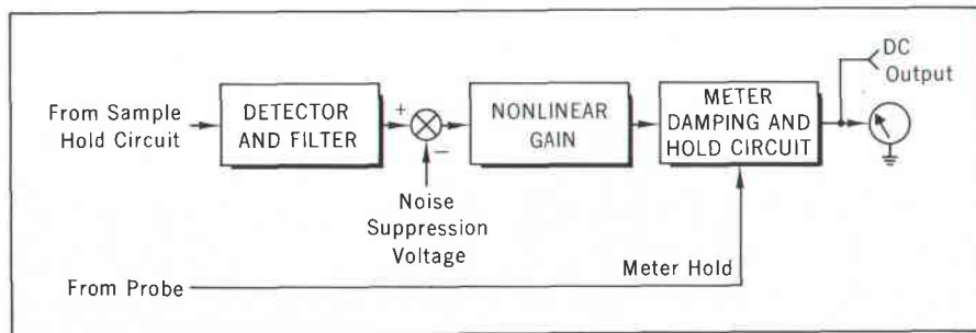
Fig. 11. Block diagram of meter circuits of sampling voltmeter. Instrument is average-responding on all voltage ranges. Damping and noise-cancellation circuits reduce effects of noise. Nonlinear gain circuit gives meter linear voltage scales.
