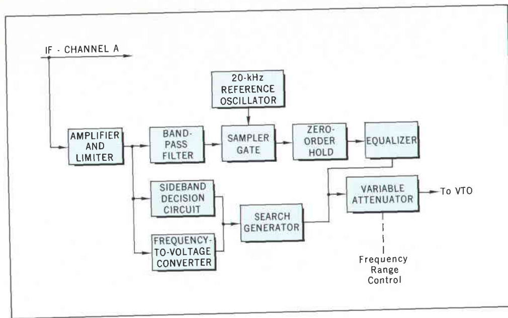
Fig. 8. Block diagram of automatic phase control (APC) circuit, which tunes and phase-locks Vector Voltmeter to channel A signal. APC loop adjusts frequency of voltage-tuned local oscillator (VTO) which generates sampling pulses for mixers, thus keeps IF at 20 kHz. APC requires only 10 ms to tune meter, and remains locked even if input frequency changes at rates up to 15 MHz/s. Sideband decision circuit ensures that f_{sig} - nf_{VTO} is always +20 kHz, never -20 kHz.
