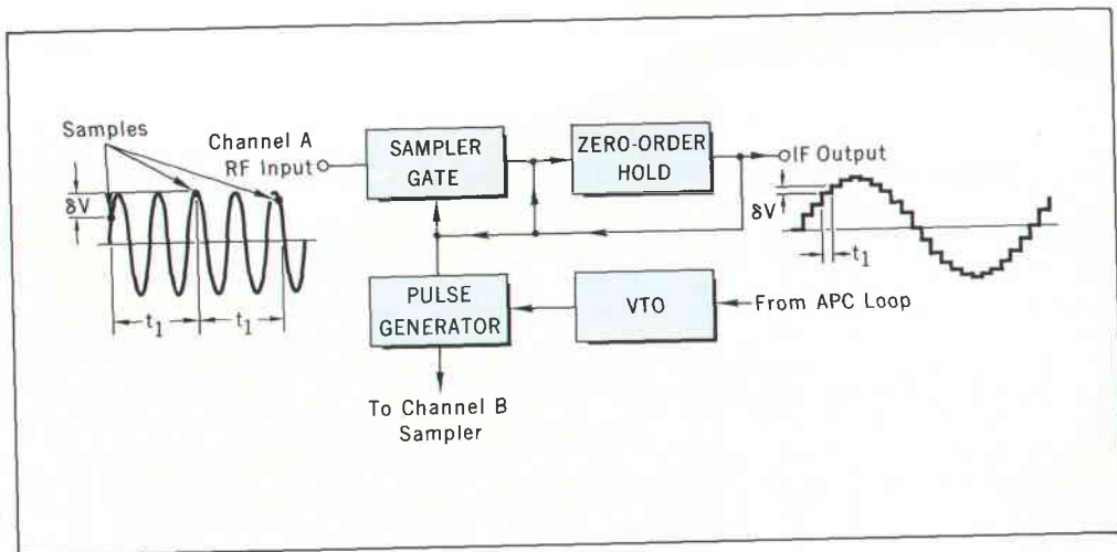
Fig. 7. Block diagram of sampling-type harmonic mixers used in new VVM. Mixers operate on stroboscopic principle, sampling RF signal at different points in cycle at successive sampling instants. RF waveforms are reconstructed in small steps at intermediate frequency: fundamental component of RF signal is transposed to 20 kHz, second harmonic to 40 kHz, and so on. Feedback keeps IF voltage equal to RF voltage.
