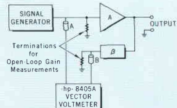
Terminations for Open-Loop Gain Measurements
