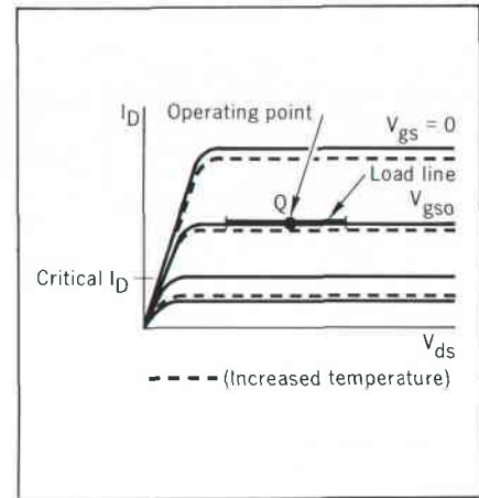
Fig. 4. Typical characteristic curves for field-effect transistor. Increase in temperature changes V_{GS0} of load line to compensate for temperature-induced changes of operating points in associated bi-polar transistors.
