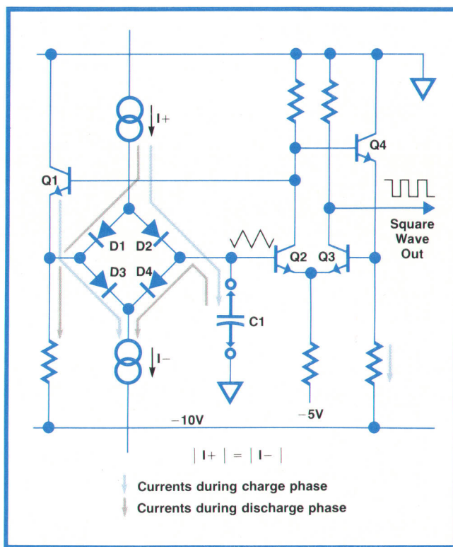
Fig. 3. Simplified diagram of the rate generator. Equal charge and discharge times of capacitor C1 result in a square wave output. Ranges are changed by switching capacitor C1; currents I_+ and I_- provide vernier control of rate.
