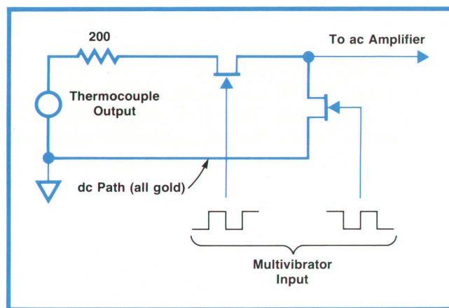
Fig. 6. Dc path in sensor is all gold to eliminate undesired thermocouples. Care was taken to assure that the two chopper FET's would remain at the same temperature to minimize drift.
