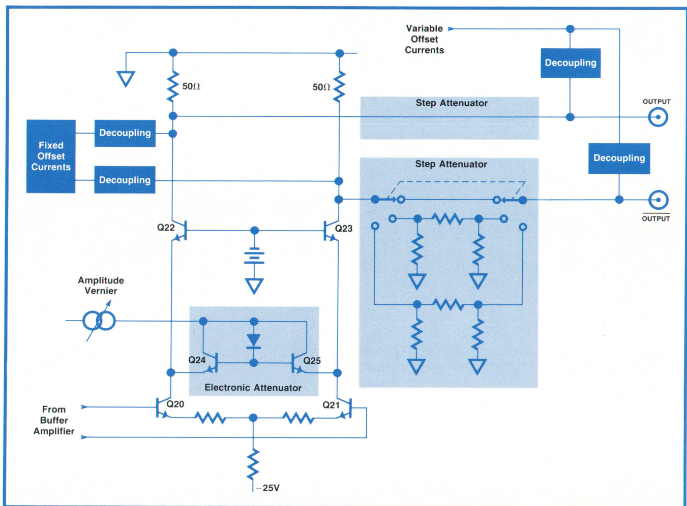
Fig. 5. Simplified diagram of the output stage. The amplifier functions as a current source, so source impedance is established by the 50 \Omega collector load resistors.
