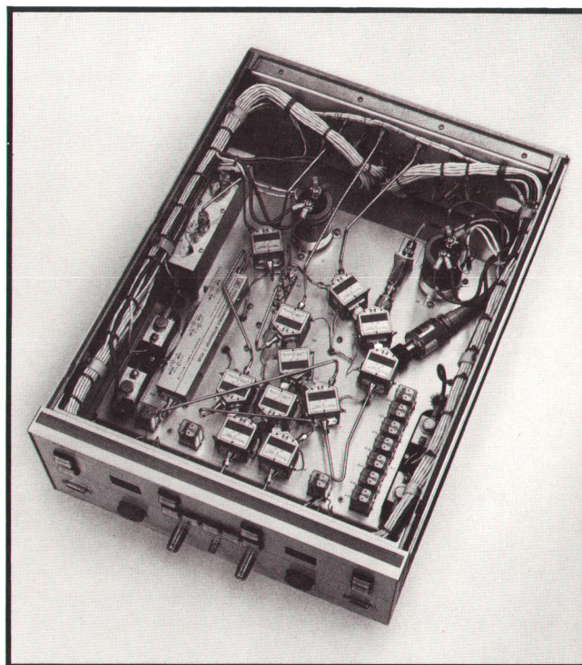
Fig. 5. Inside the RF test head are a down-converting mixer, a peak detector, a thermistor mount, a programmable attenuator and programmable RF switches.
