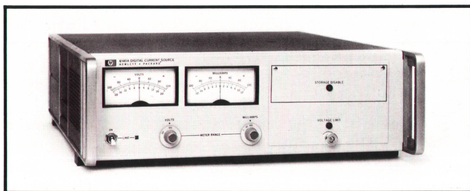
Fig. 1. Model 6140A Digitally-Programmable Current Source supplies current accurately at levels up to \pm 160 mA in response to digital input commands. It accepts various logic levels and formats according to interface circuit boards that are installed through the removable panel on the front-panel.
