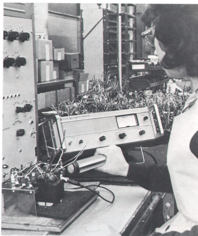
Ultrasonic inspection of high-voltage filament transformers for corona, using new Model 4950A Ultrasonic Translator. Translator alarm light indicates too much corona. Test voltage is 3.5 kV.
