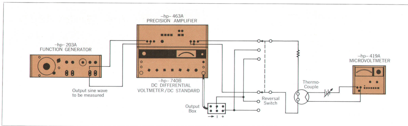
Fig. 4. Measuring the output of an oscillator using a precision amplifier as a buffer with an indirectly-heated thermocouple.
