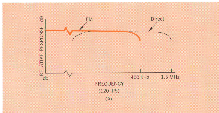
Fig. 2. Frequency response in the FM mode and Direct mode at a tape speed of 120 ips (a) and 3 \frac{3}{4} ips (b). In the FM mode, bandwidth is exchanged for dc response and freedom from dropouts.
