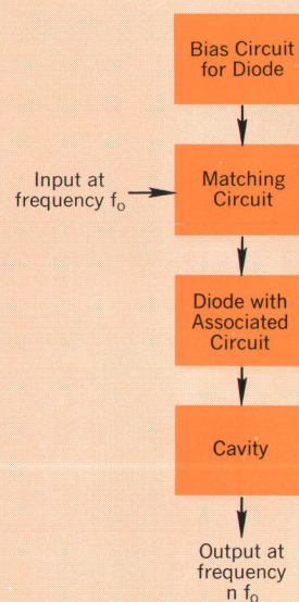
Fig. 1. General frequency multiplier block diagram.
