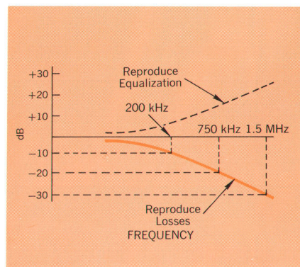
Fig. 5. Losses in the record/reproduce process must be made up by equalization in the reproduce system.
