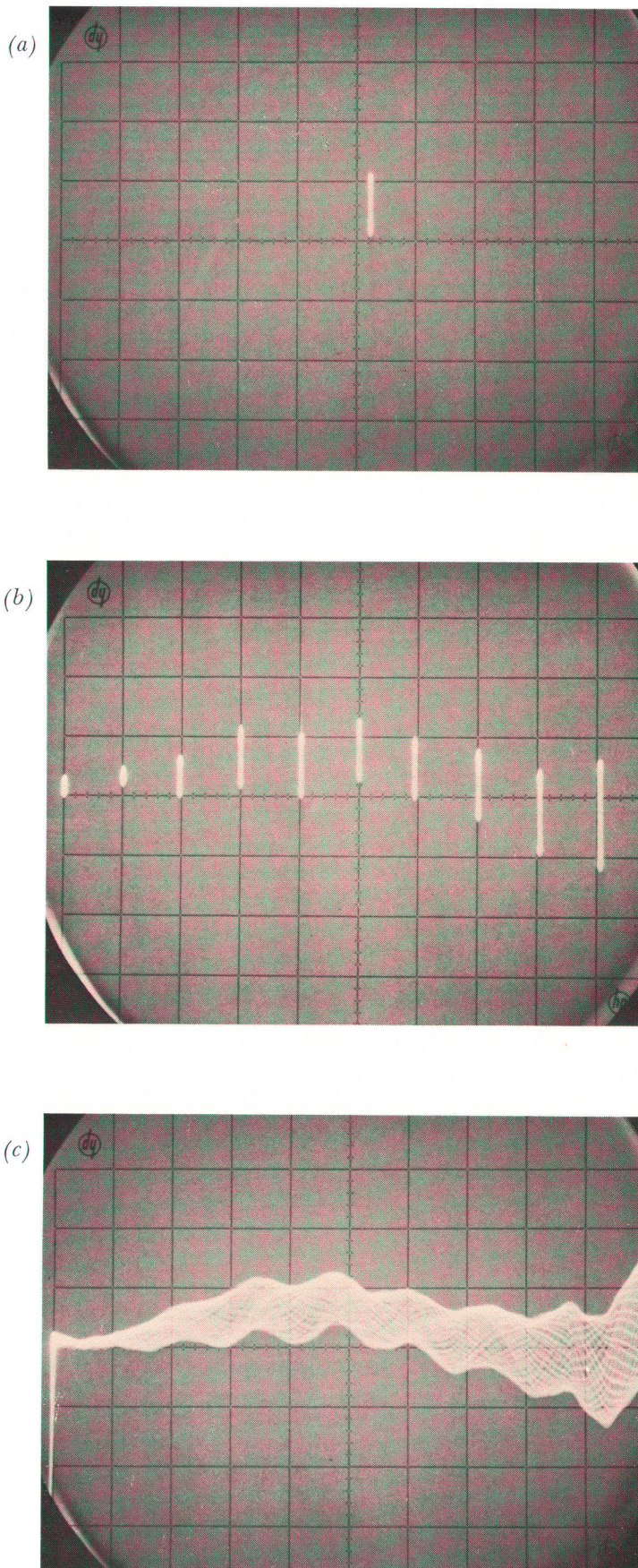
Fig. 2. Oscillograms made with setup of Fig. 1, showing measurement of SWR of a load.
