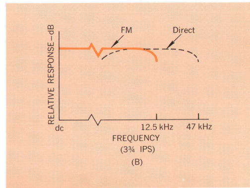
Fig. 2. Frequency response in the FM mode and Direct mode at a tape speed of 120 ips (a) and 3 \frac{3}{4} ips (b). In the FM mode, bandwidth is exchanged for dc response and freedom from dropouts.
