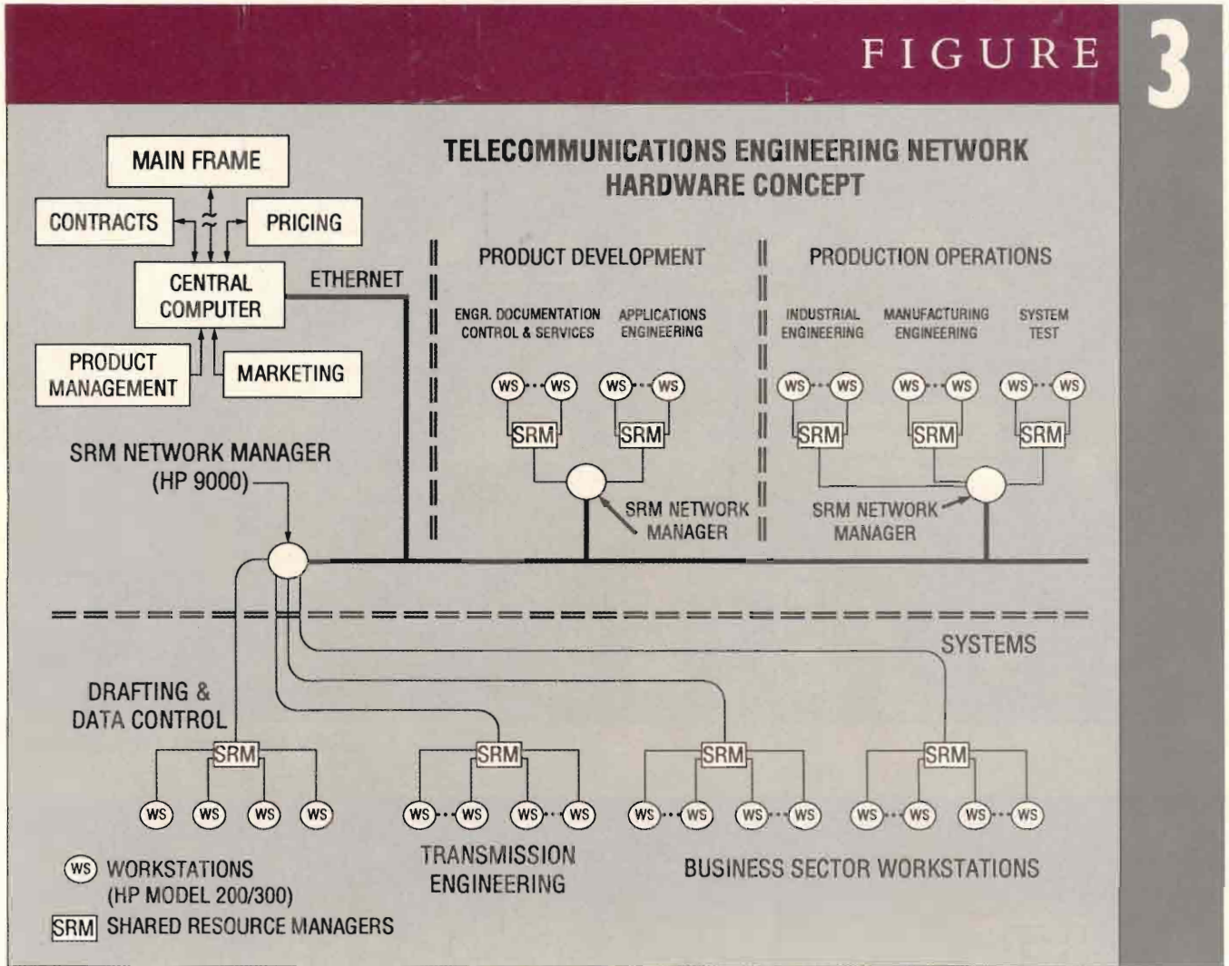
TEN System Layout
