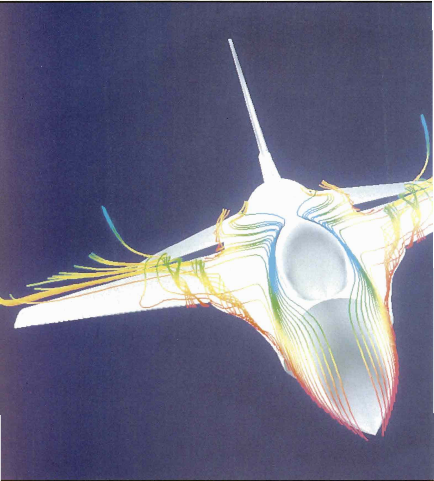
This photo, courtesy of Sterling Software and NASA/Ames Research, shows the simulated flow field around the F-16 A.
